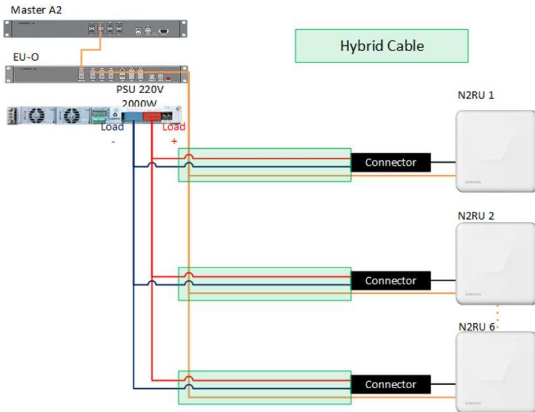
Figure 1. Hybrid Cable Configuration
