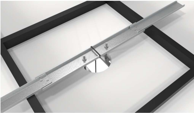
Figure 40. Placing Bracket 2
