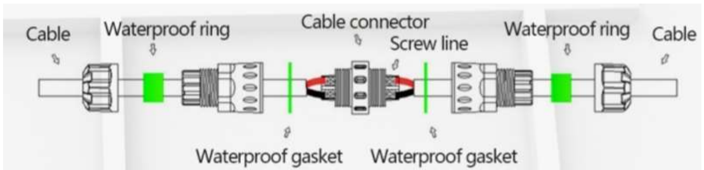
Figure 2. Cable Connector Diagram
