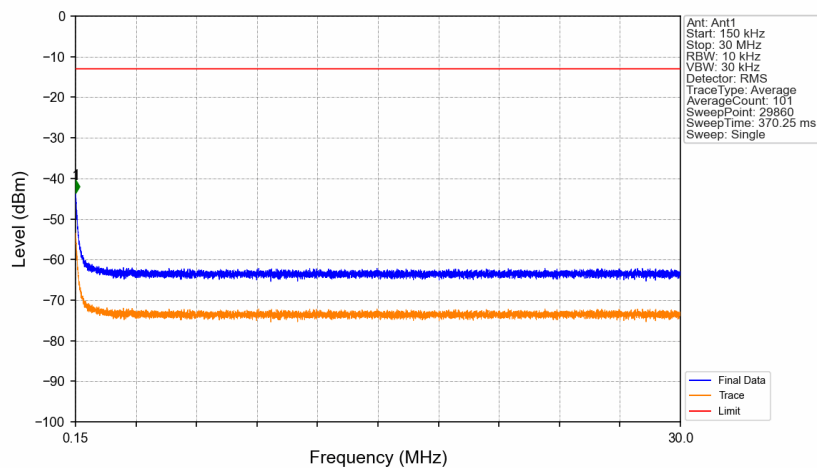
Band14_765.5MHz_AWGN_SISO_Ant1_NTNV
