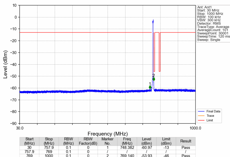
Band14_765.5MHz_AWGN_SISO_Ant1_NTNV
