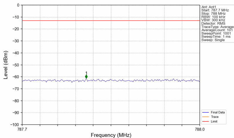
Band14_760.5MHz_AWGN_SISO_Ant1_NTNV_AGC
