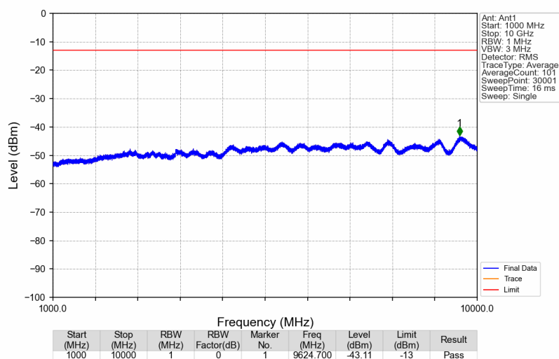
Band14_765.5MHz_AWGN_SISO_Ant1_NTNV
