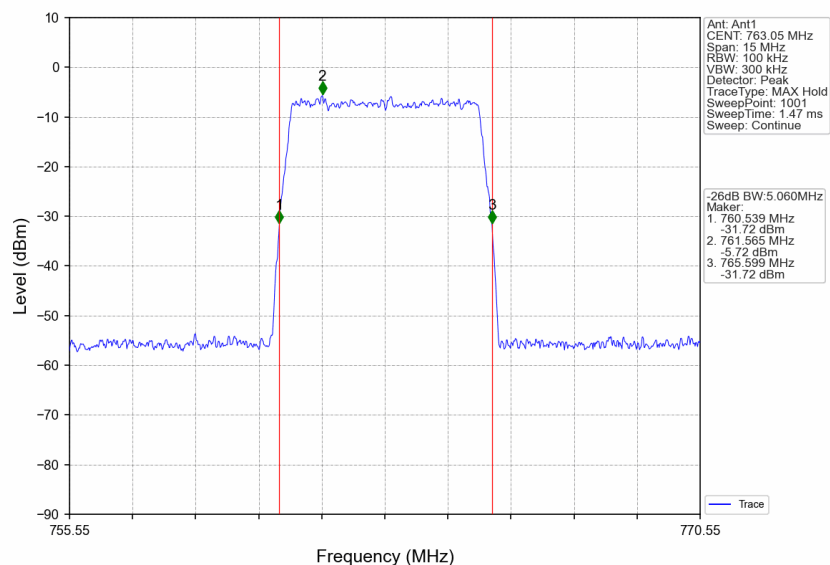
Band14_763.05MHz_AWGN_SISO_Ant1_NTNV_Input_AGC+3
