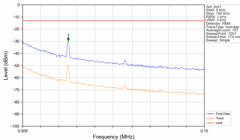
Band14_765.5MHz_AWGN_SISO_Ant1_NTNV
