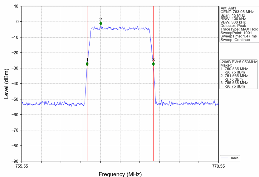
Band14_763.05MHz_AWGN_SISO_Ant1_NTNV_Input_AGC+3
