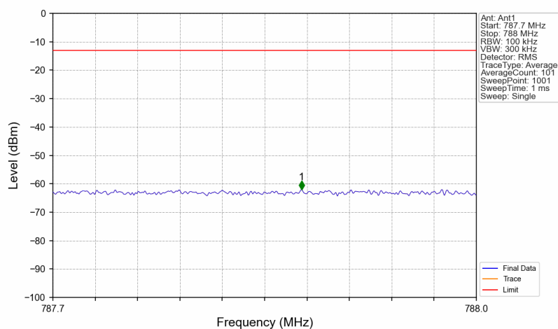
Band14_760.5MHz_AWGN_SISO_Ant1_NTNV_AGC+3
