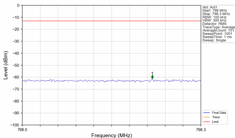
Band14_765.5MHz_AWGN_SISO_Ant1_NTNV_AGC
