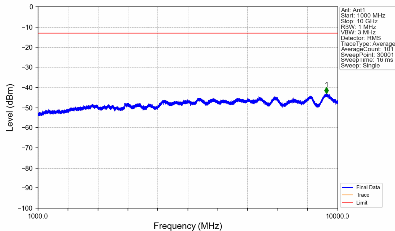
Band71_619.5MHz_AWGN_SISO_Ant1_NTNV
