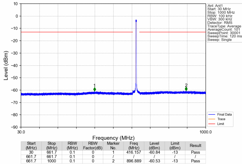
Band71_634.5MHz_AWGN_SISO_Ant1_NTNV
