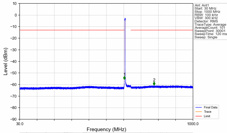
Band71_619.5MHz_AWGN_SISO_Ant1_NTNV
