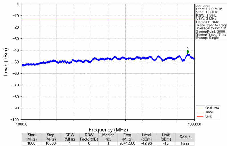
Band71_634.5MHz_AWGN_SISO_Ant1_NTNV
