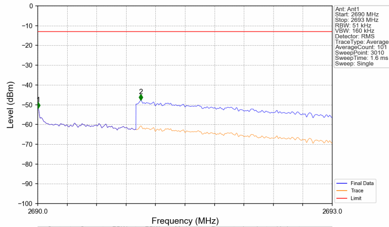
Band41_2687.5MHz_AWGN_SISO_Ant1_NTNV_AGC
