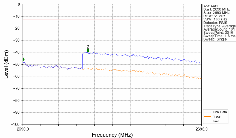
Band41_2687.5MHz_AWGN_SISO_Ant1_NTNV_AGC+3
