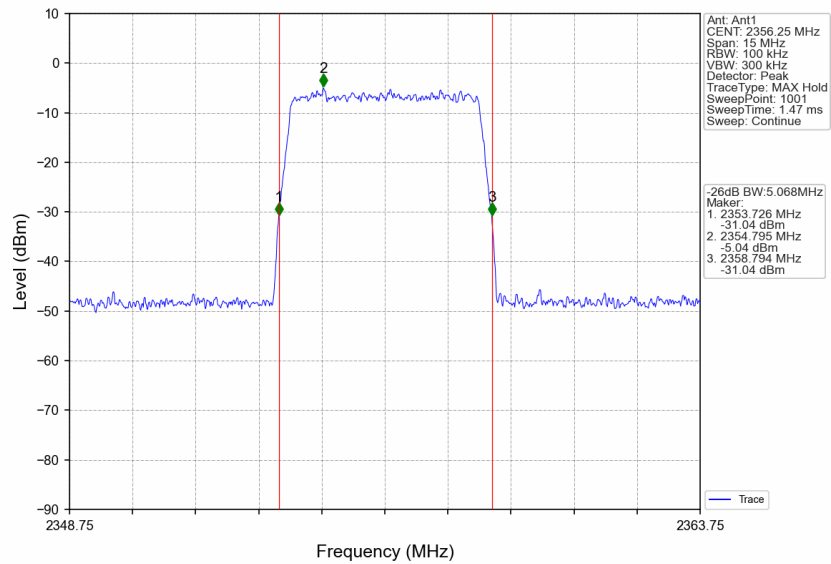
Band30_2356.25MHz_AWGN_SISO_Ant1_NTNV_Input_AGC+3
