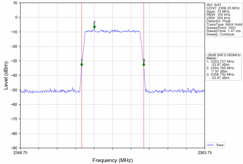
Band30_2356.25MHz_AWGN_SISO_Ant1_NTNV_Input_AGC+3
