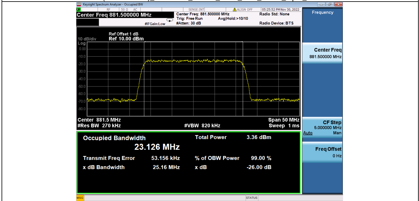
N26(869-894MHz)_881.5MHz_AWGN_SISO_Ant1_NTNV_Input_AGC+3
