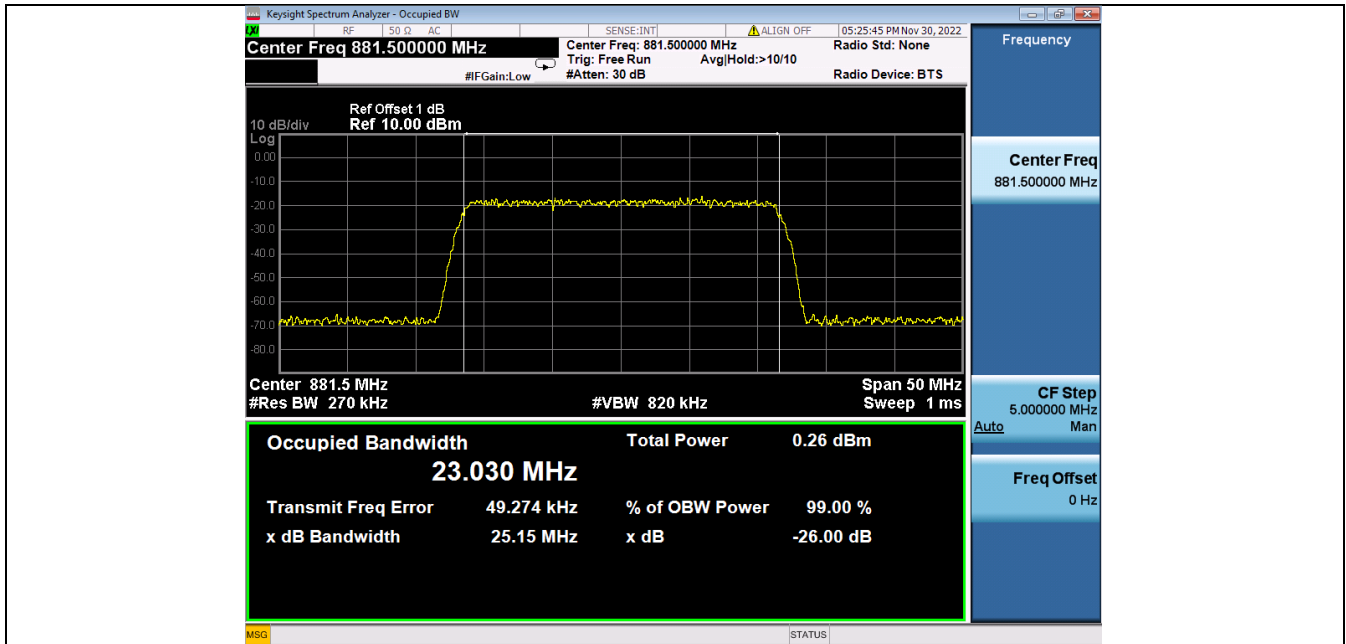
N26(869-894MHz)_881.5MHz_AWGN_SISO_Ant1_NTNV_Input_AGC+3
