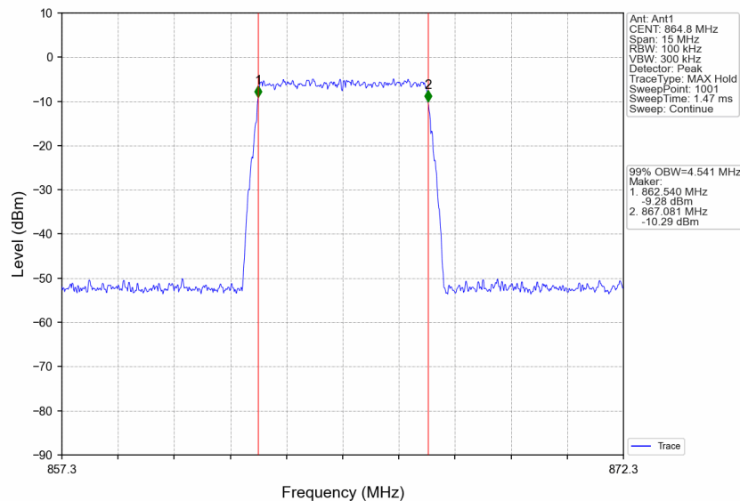
Band26a_864.8MHz_AWGN_SISO_Ant1_NTNV_Input_AGC+3
