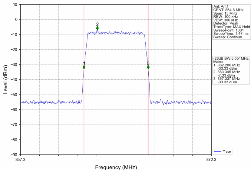
Band26a_864.8MHz_AWGN_SISO_Ant1_NTNV_Input_AGC+3
