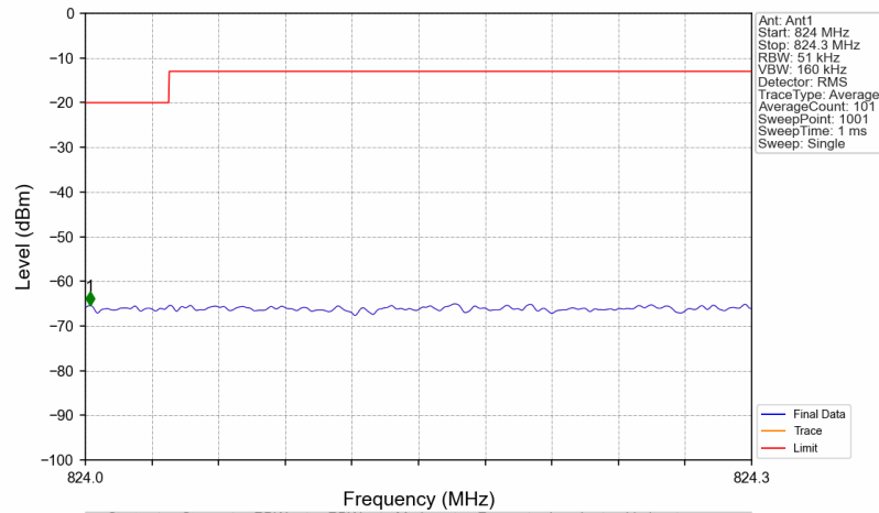
Band26a_866.5MHz_AWGN_SISO_Ant1_NTNV_AGC
