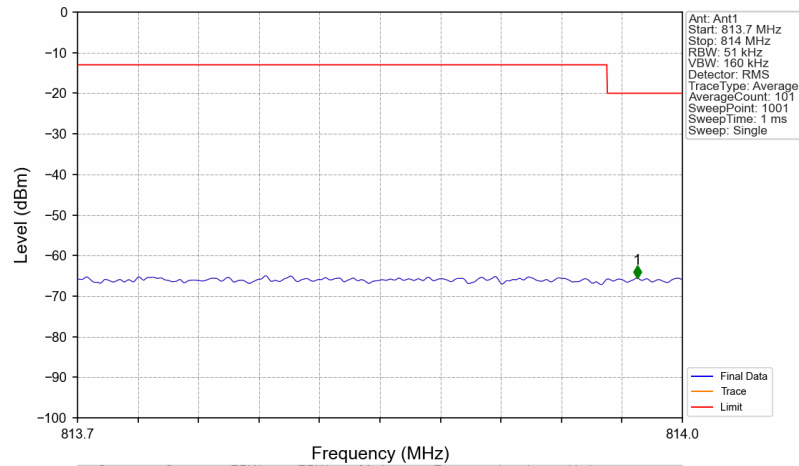
Band26a_864.5MHz_AWGN_SISO_Ant1_NTNV_AGC
