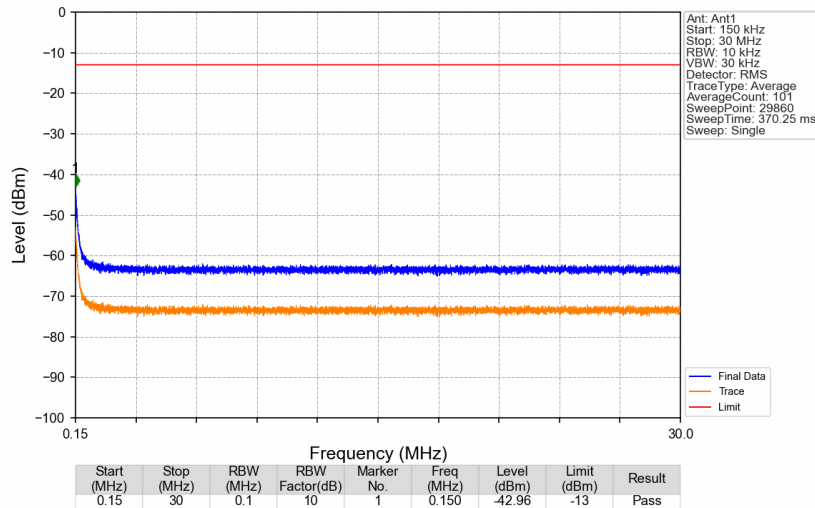
Band13_753.5MHz_AWGN_SISO_Ant1_NTNV
