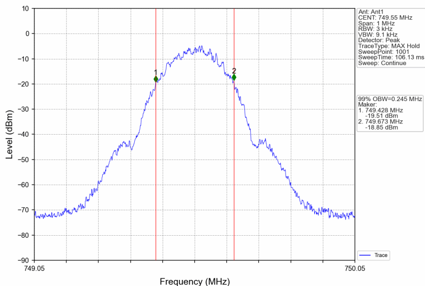
Band13_749.55MHz_GMSK_SISO_Ant1_NTNV_Input_AGC+3
