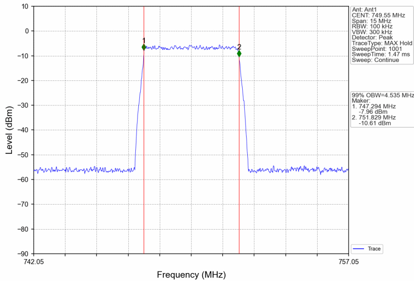
Band13_749.55MHz_AWGN_SISO_Ant1_NTNV_Input_AGC+3
