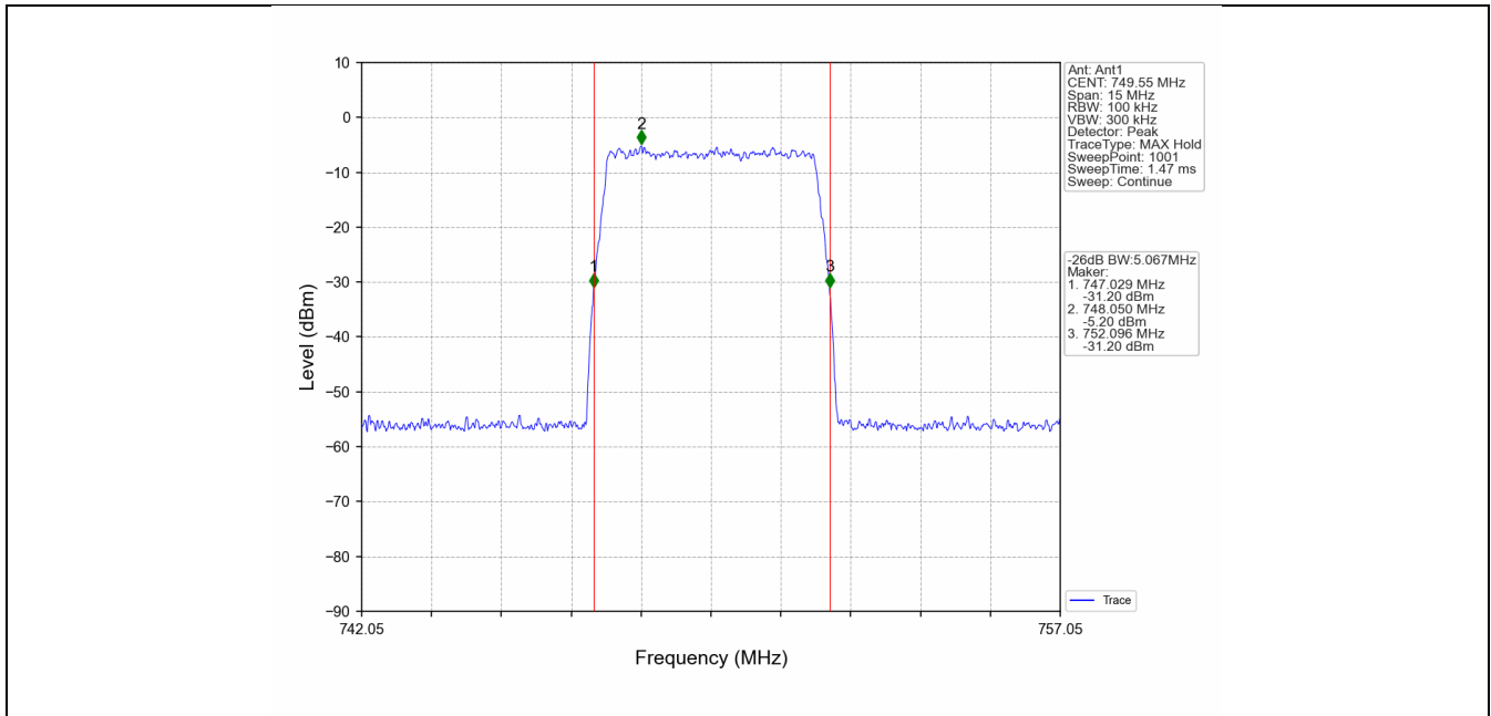
Band13_749.55MHz_AWGN_SISO_Ant1_NTNV_Input_AGC+3
