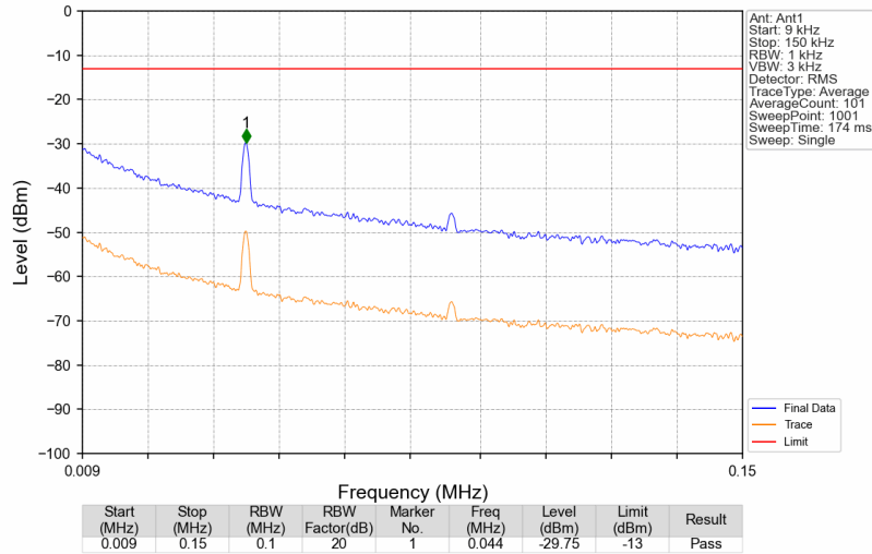
Band13_753.5MHz_AWGN_SISO_Ant1_NTNV
