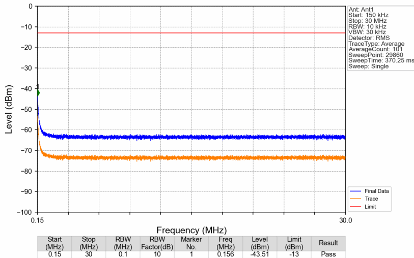
Band14_765.5MHz_AWGN_SISO_Ant1_NTNV
