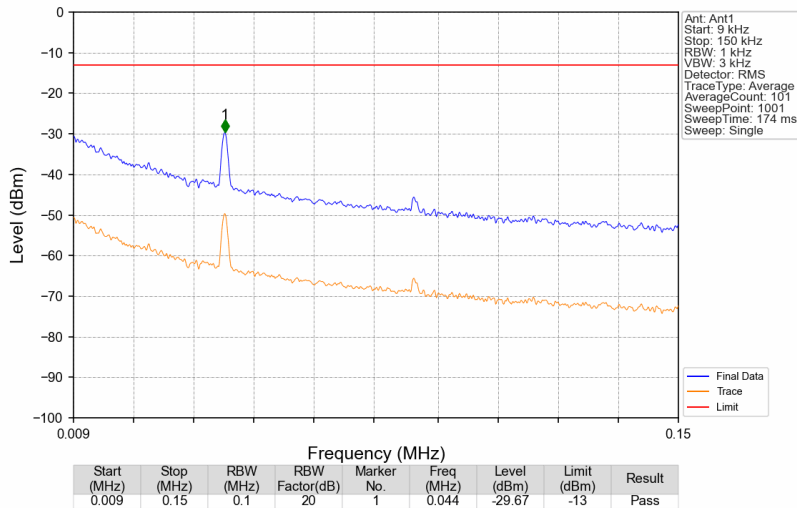
Band14_765.5MHz_AWGN_SISO_Ant1_NTNV
