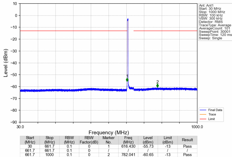
Band71_619.5MHz_AWGN_SISO_Ant1_NTNV
