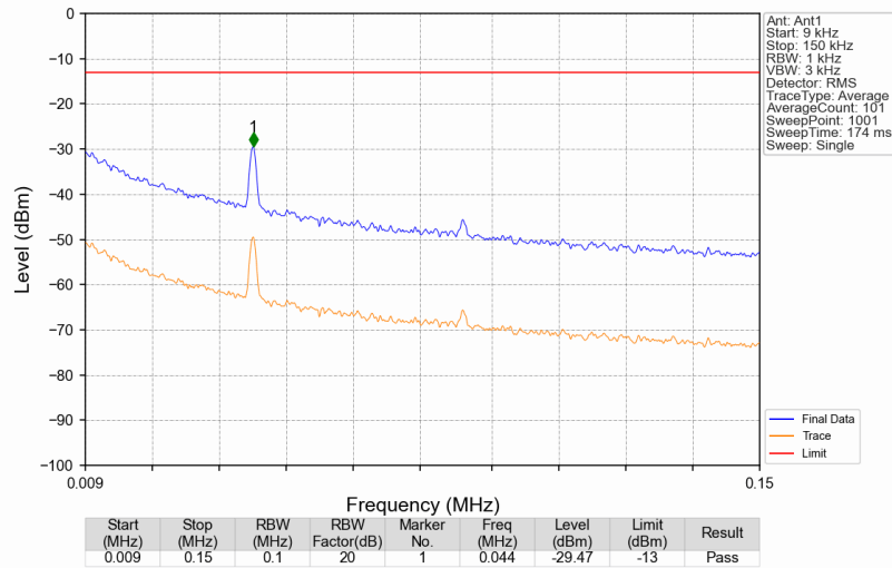
Band71_634.5MHz_AWGN_SISO_Ant1_NTNV
