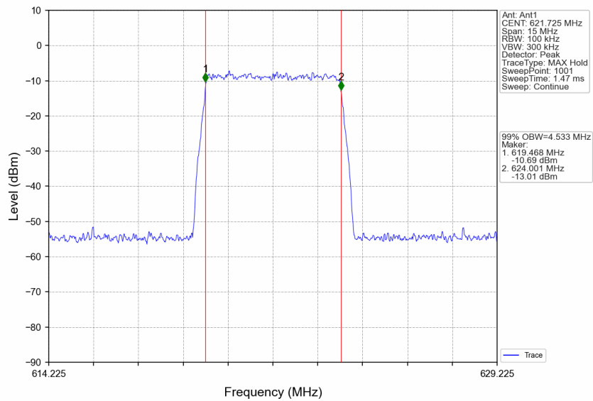
Band71_621.725MHz_AWGN_SISO_Ant1_NTNV_Input_AGC+3
