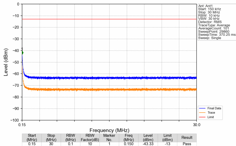
Band71_634.5MHz_AWGN_SISO_Ant1_NTNV
