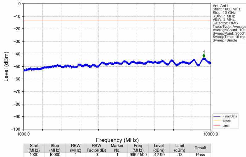
Band71_619.5MHz_AWGN_SISO_Ant1_NTNV
