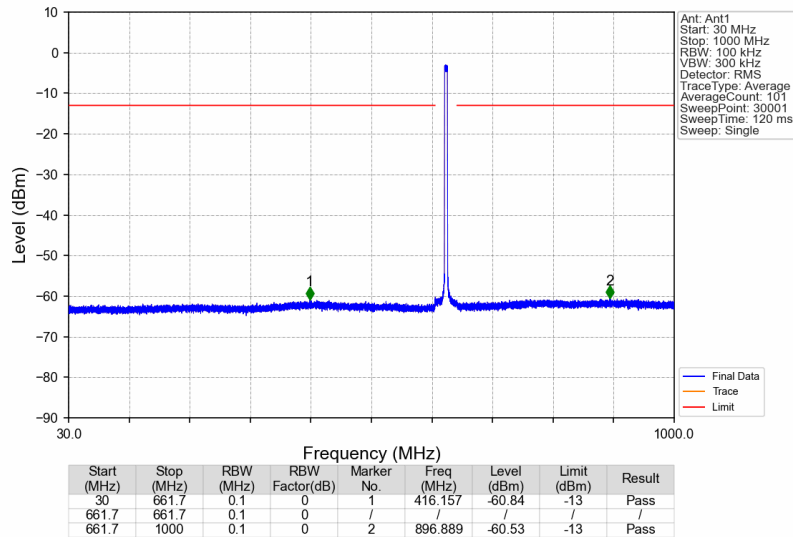
Band71_634.5MHz_AWGN_SISO_Ant1_NTNV
