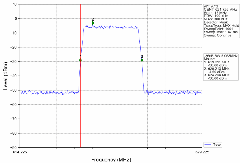
Band71_621.725MHz_AWGN_SISO_Ant1_NTNV_Input_AGC+3
