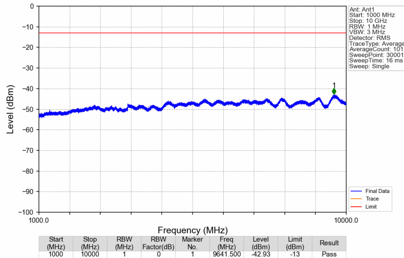
Band71_634.5MHz_AWGN_SISO_Ant1_NTNV
