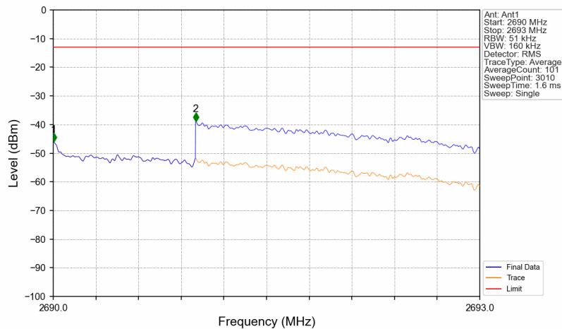
Band41_2687.5MHz_AWGN_SISO_Ant1_NTNV_AGC+3
