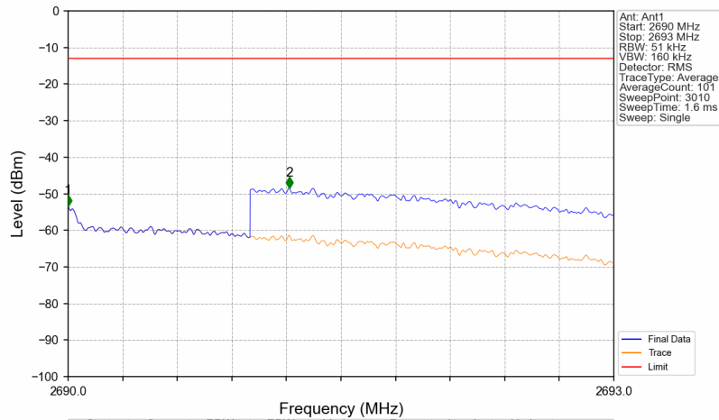
Band41_2687.5MHz_AWGN_SISO_Ant1_NTNV_AGC
