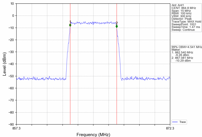
Band26a_864.8MHz_AWGN_SISO_Ant1_NTNV_Input_AGC+3
