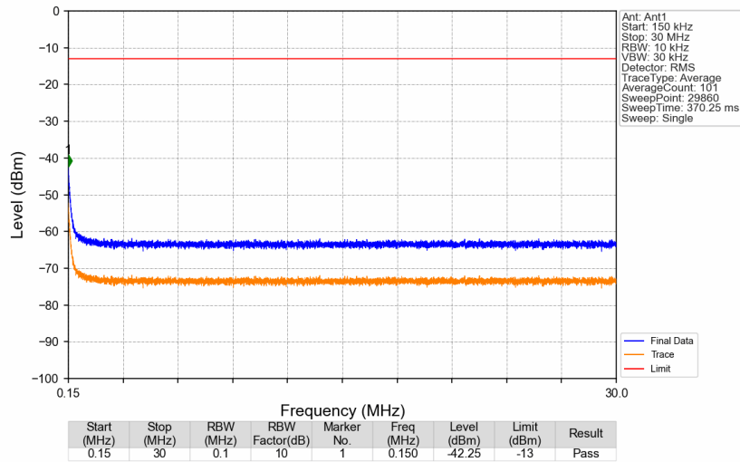
Band26a_865.5MHz_AWGN_SISO_Ant1_NTNV
