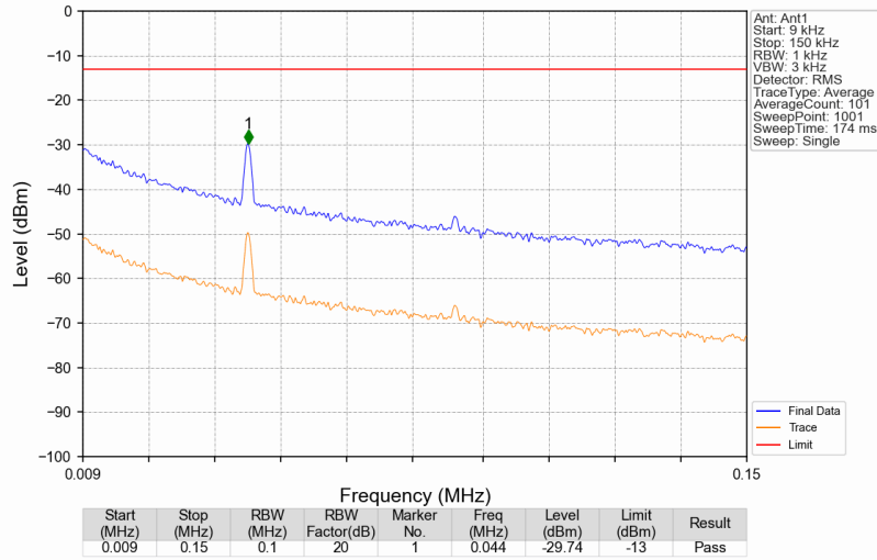
Band26a_865.5MHz_AWGN_SISO_Ant1_NTNV
