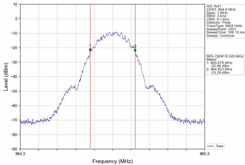
Band26a_864.8MHz_GMSK_SISO_Ant1_NTNV_Input_AGC+3
