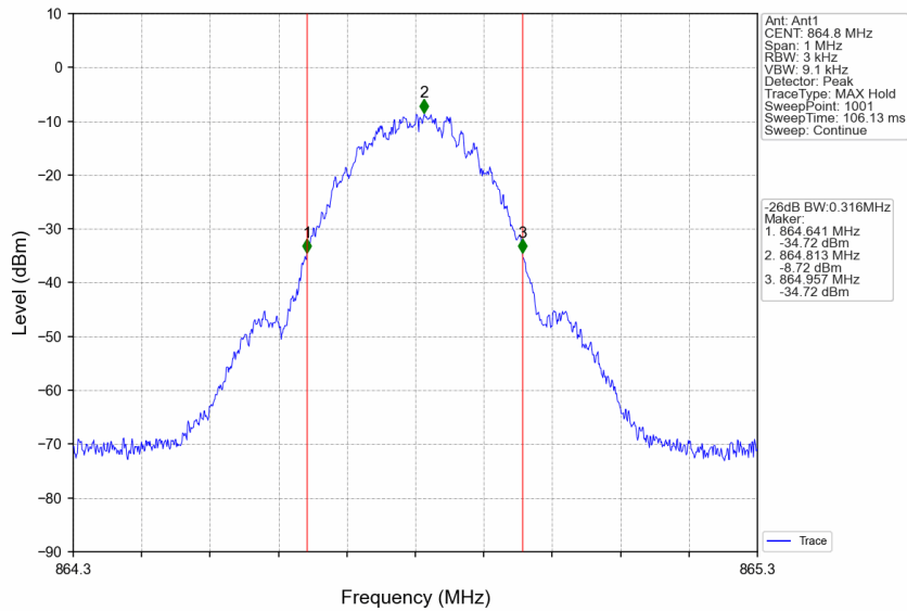
Band26a_864.8MHz_GMSK_SISO_Ant1_NTNV_Input_AGC+3
