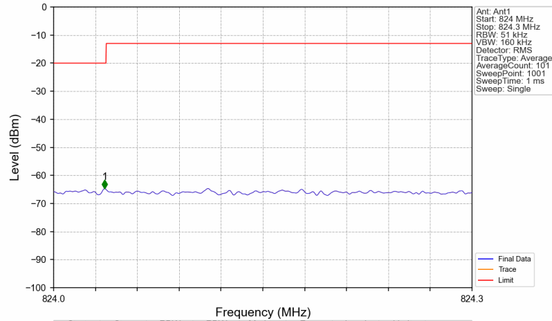
Band26a_866.5MHz_AWGN_SISO_Ant1_NTNV_AGC
