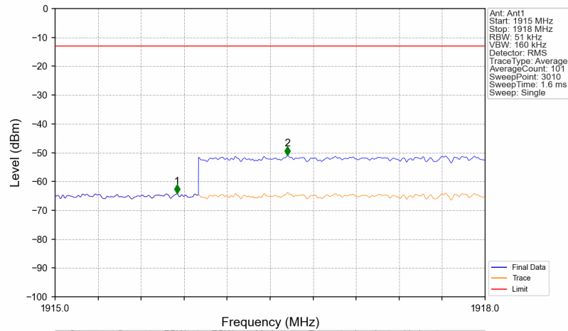
Band25_1992.5MHz_AWGN_SISO_Ant1_NTNV_AGC
