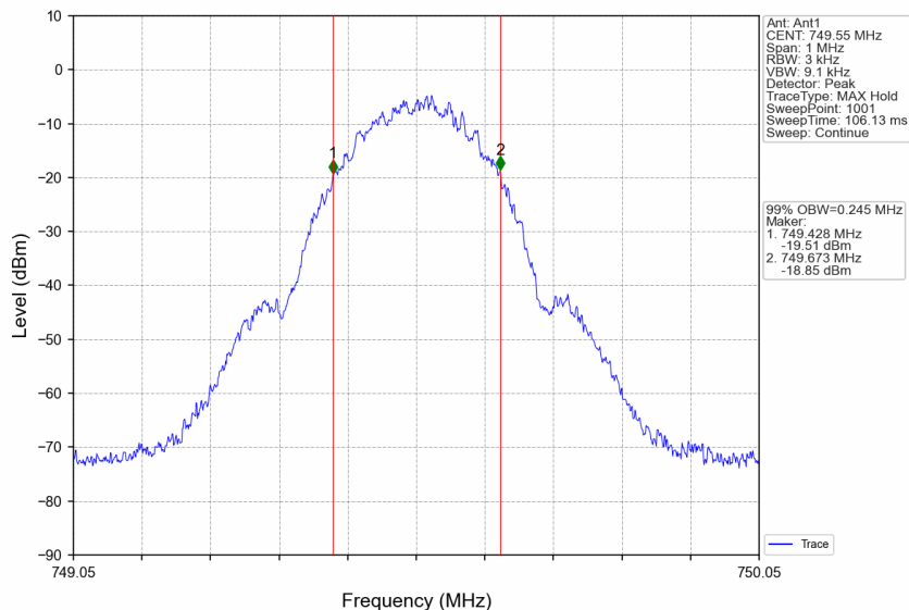
Band13_749.55MHz_GMSK_SISO_Ant1_NTNV_Input_AGC+3
