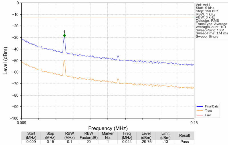
Band13_753.5MHz_AWGN_SISO_Ant1_NTNV
