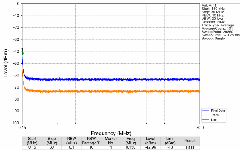
Band13_753.5MHz_AWGN_SISO_Ant1_NTNV
