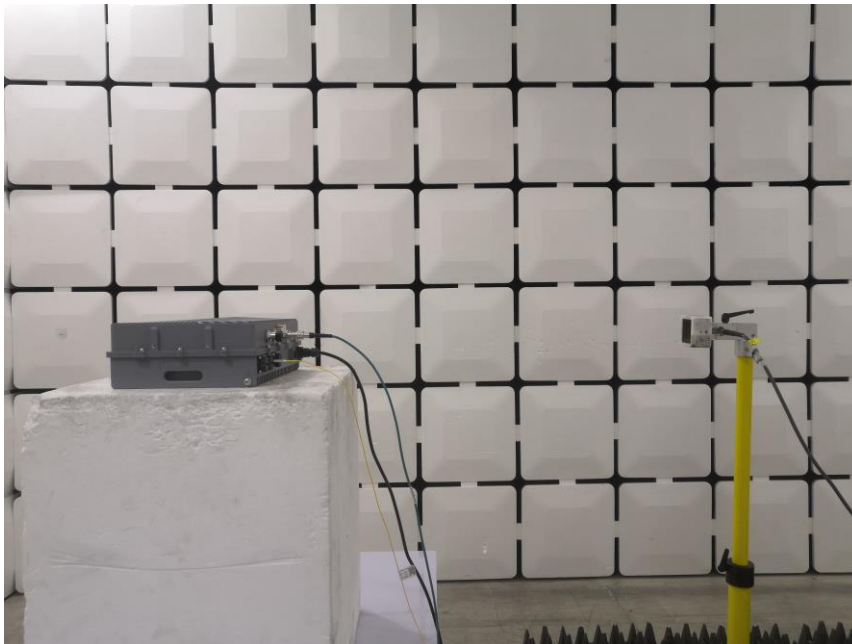
Radiated Spurious Emissions (Above 18GHz)
