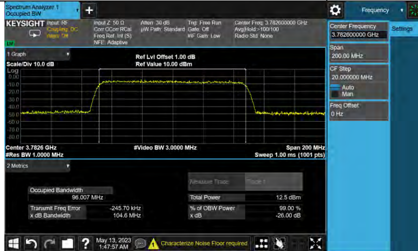
Bandn77a_3782.6MHz_AWGN_SISO_Ant1_NTNV_Input_AGC+3
