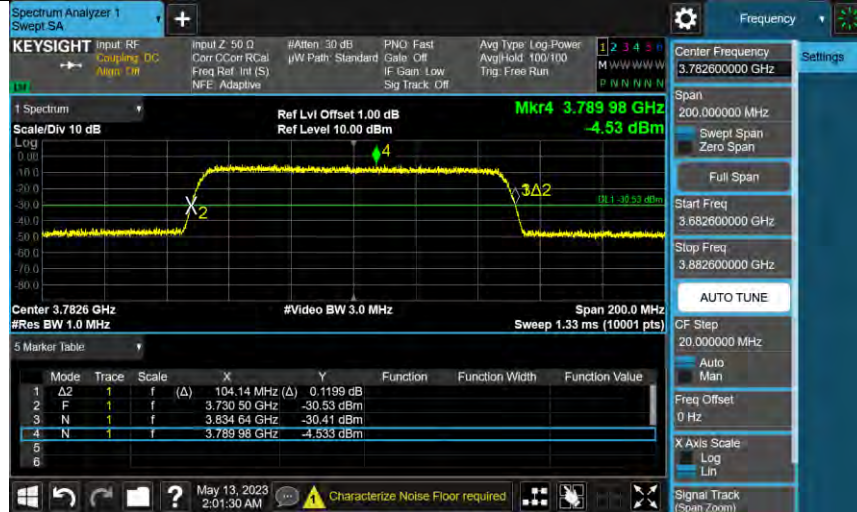
Bandn77a_3782.6MHz_AWGN_SISO_Ant1_NTNV_Input_AGC+
