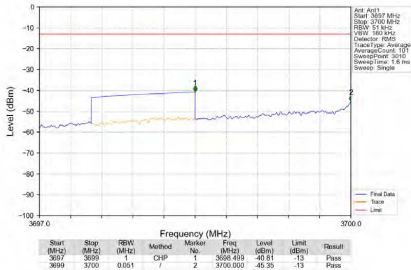
Bandn77a_3702.5MHz_AWGN_SISO_Ant1_NTNV_AGC+3
