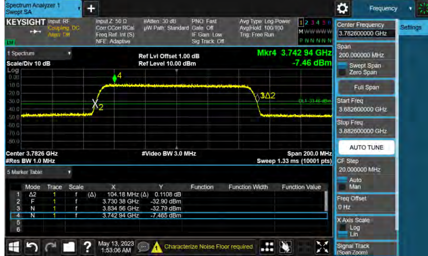
Bandn77a_3782.6MHz_AWGN_SISO_Ant1_NTNV_Input_AGC+
