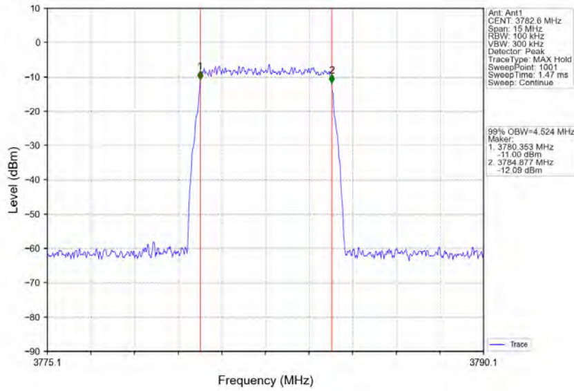
Bandn77a_3782.6MHz_AWGN_SISO_Ant1_NTNV_Input_AGC+3
