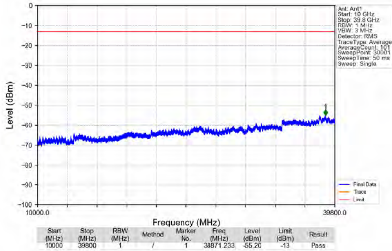
Bandn77a_3702.5MHz_AWGN_SISO_Ant1_NTNV
