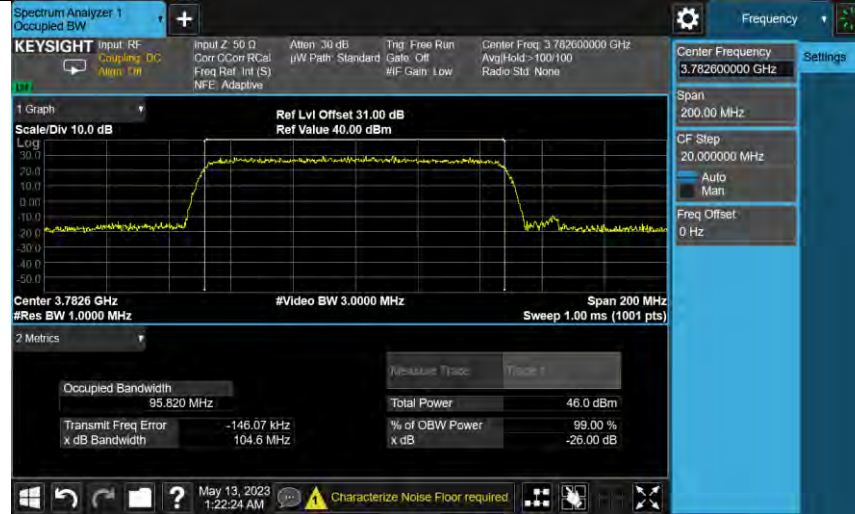
Bandn77a_3782.6MHz_AWGN_SISO_Ant1_NTNV_Output_AGC+3
