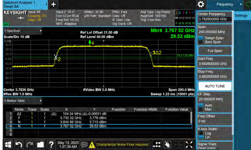
Bandn77a_3782.6MHz_AWGN_SISO_Ant1_NTNV_Output_AGC+3
