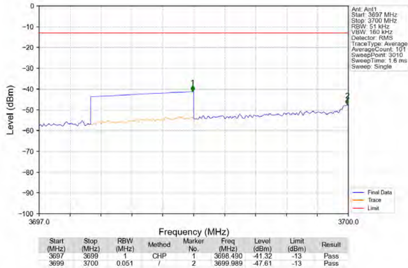
Bandn77a_3702.5MHz_AWGN_SISO_Ant1_NTNV_AGC
