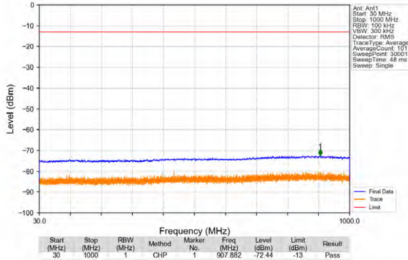
Bandn77a_3702.5MHz_AWGN_SISO_Ant1_NTNV
