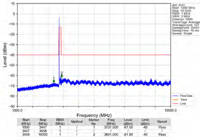
Bandn78e_3452.5MHz_AWGN_SISO_Ant1_NTNV
