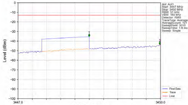
Bandn78e_3452.5MHz_AWGN_SISO_Ant1_NTNV_AGC
