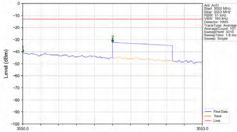
Bandn78e_3547.5MHz_AWGN_SISO_Ant1_NTNV_AGC
