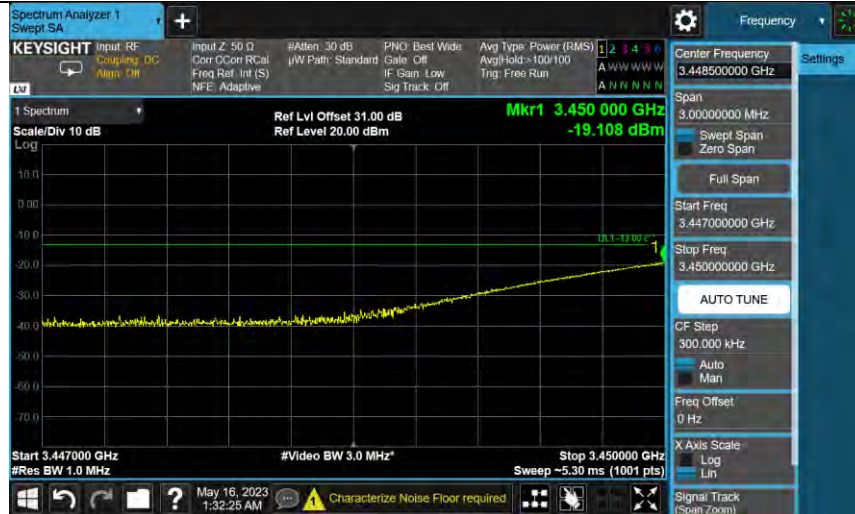
Bandn78e_3500MHz_AWGN_SISO_Ant1_NTNV_AGC+3
