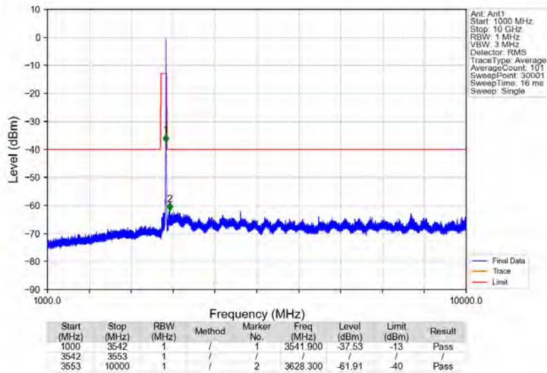
Bandn78e_3547.5MHz_AWGN_SISO_Ant1_NTNV
