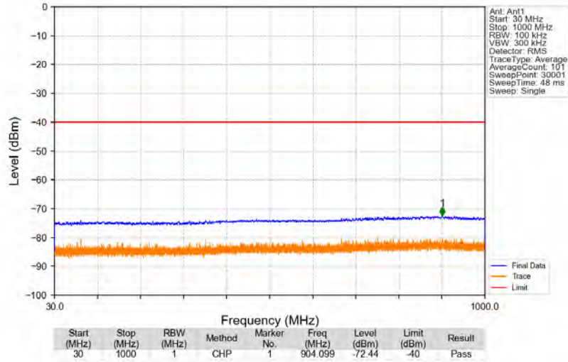
Bandn78e_3547.5MHz_AWGN_SISO_Ant1_NTNV
