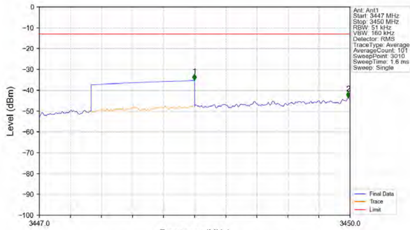
Bandn78e_3452.5MHz_AWGN_SISO_Ant1_NTNV_AGC+3
