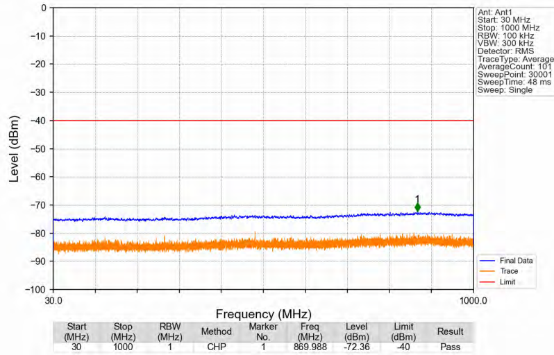
Bandn78e_3452.5MHz_AWGN_SISO_Ant1_NTNV
