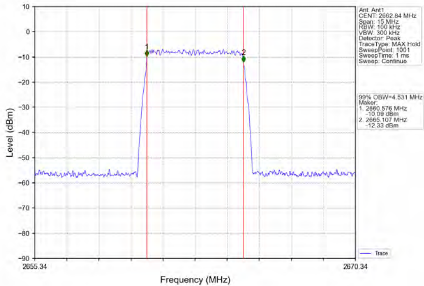
Band41_2662.84MHz_AWGN_SISO_Ant1_NTNV_Input_AGC+3
