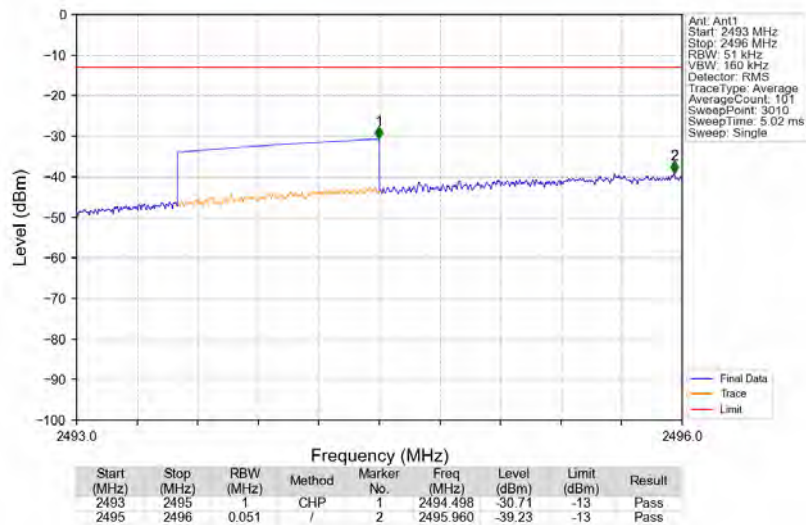
Band41_2498.5MHz_AWGN_SISO_Ant1_NTNV_AGC+3
