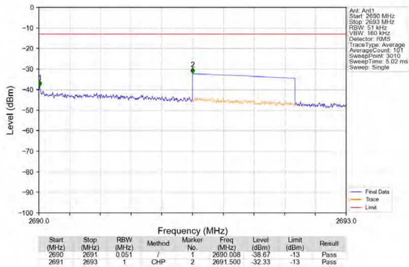
Band41_2687.5MHz_AWGN_SISO_Ant1_NTNV_AGC+3
