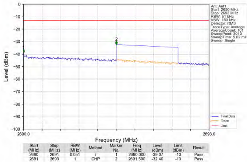
Band41_2687.5MHz_AWGN_SISO_Ant1_NTNV_AGC
