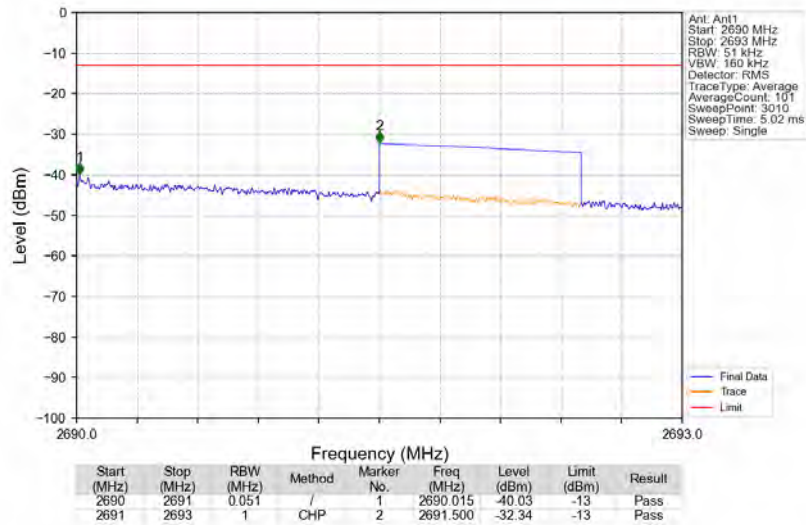
Band41_2687.5MHz_AWGN_SISO_Ant1_NTNV_AGC+3
