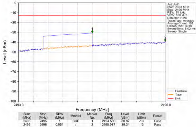
Band41_2498.5MHz_AWGN_SISO_Ant1_NTNV_AGC
