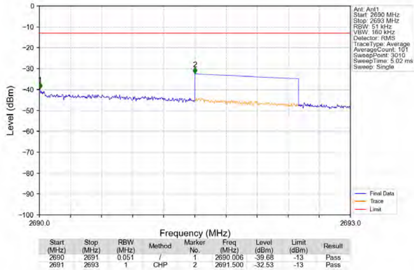
Band41_2687.5MHz_AWGN_SISO_Ant1_NTNV_AGC
