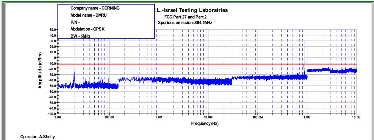
Figure 472: Spurious Emissions at Antenna Terminal QPSK, 864.5MHz, B.W. 5MHz
