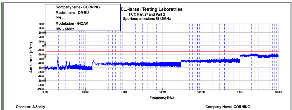
Figure 465: Spurious Emissions at Antenna Terminal 64QAM, 891.5MHz, B.W. 5MHz
