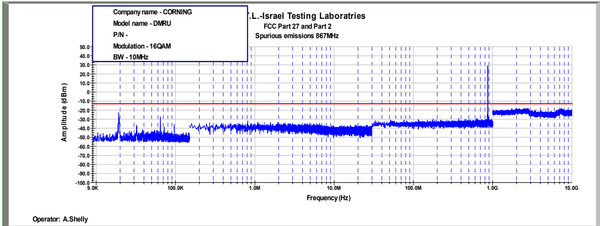
Figure 457: Spurious Emissions at Antenna Terminal 16QAM, 867.0MHz, B.W. 10MHz
