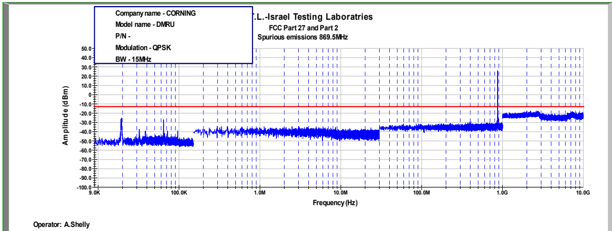
Figure 478: Spurious Emissions at Antenna Terminal QPSK, 869.5MHz, B.W. 15MHz
