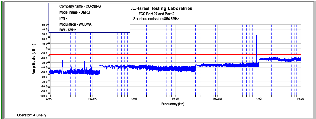
Figure 481: Spurious Emissions at Antenna Terminal WCDMA, 864.5MHz, B.W. 5MHz
