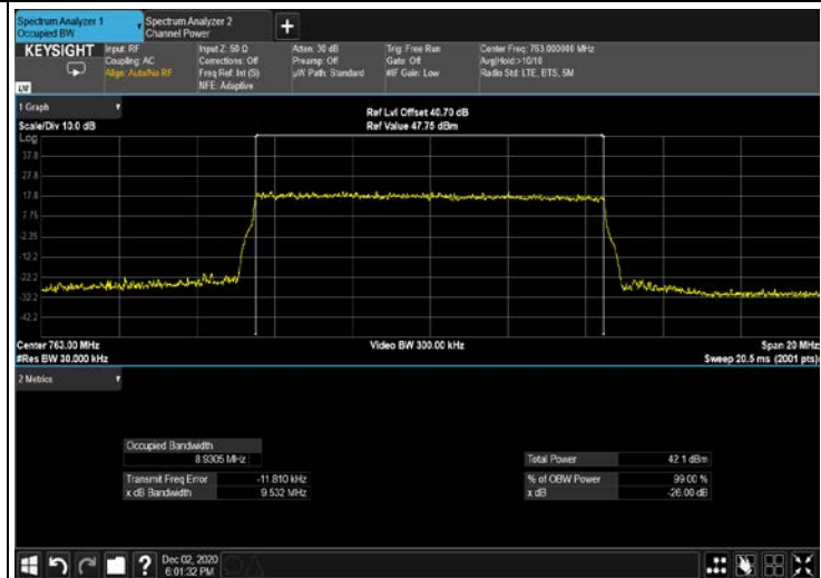
Figure 355: 16QAM 10MHz; 763.0MHz output 4G
