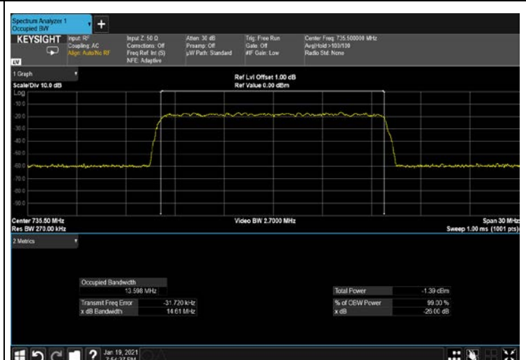
Figure 258: 256QAM 15MHz B.W; 735.5MHz, 30kHz INPUT
