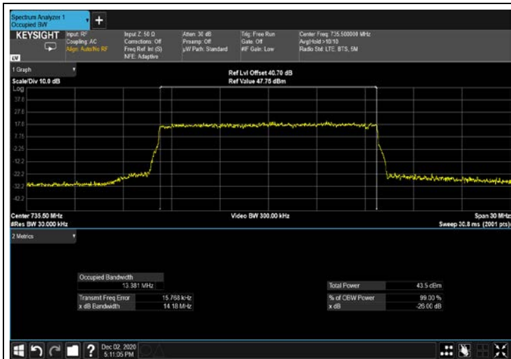
Figure 356: 16QAM 15MHz B.W; 735.5MHz output 4G
