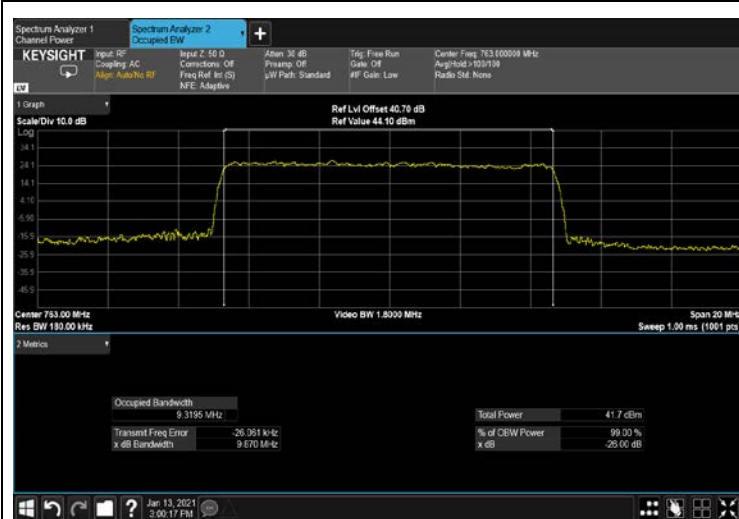
Figure 297: 64QAM 10MHz B.W; 763.0MHz, 15kHz OUTPUT
