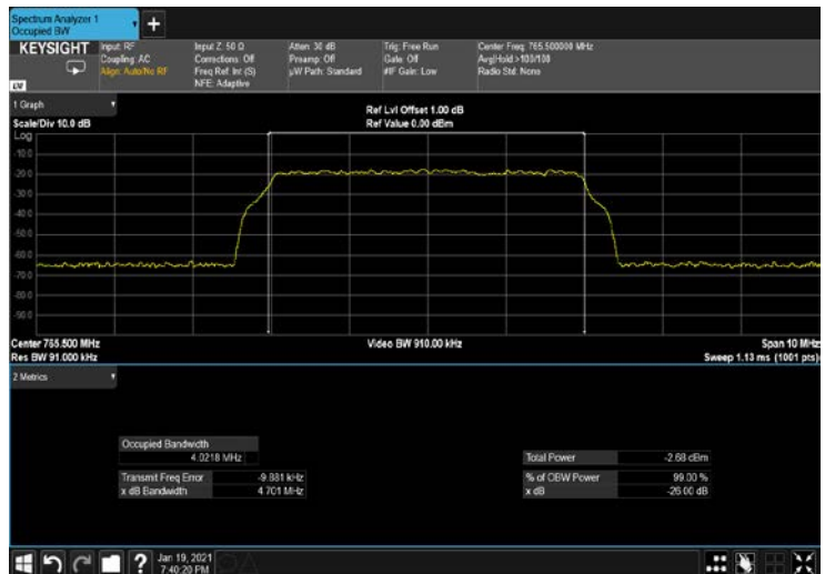
Figure 250: 256QAM 5MHz B.W; 765.5MHz, 30kHz INPUT
