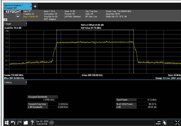
Figure 357: 64QAM 5MHz B.W; 730.5MHz output 4G
