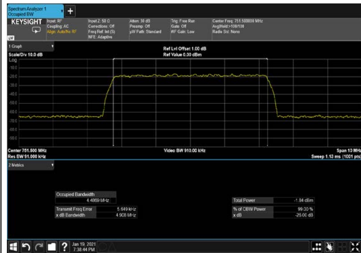
Figure 247: 256QAM 5MHz; 751.5MHz B.W, 15kHz INPUT
