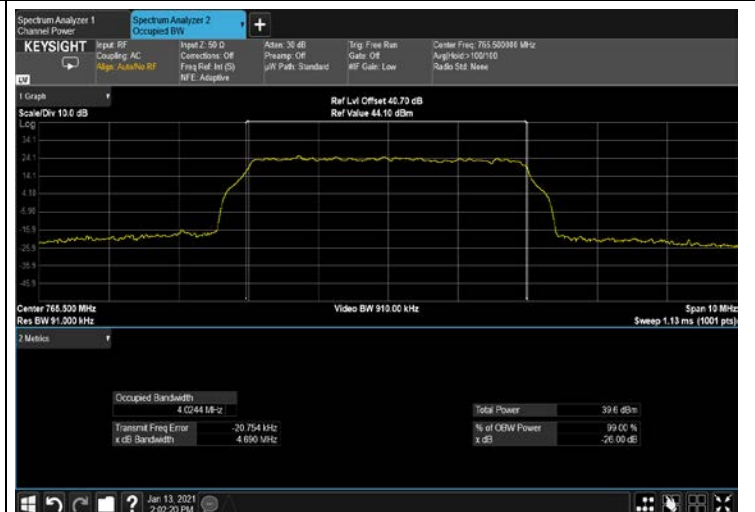
Figure 306: 256QAM 5MHz B.W; 765.5MHz, 30kHz OUTPUT
