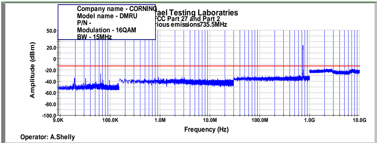
Figure 384: Spurious Emissions at Antenna Terminal 16QAM, 735.5MHz, B.W. 15MHz, Sub Carrier 30kHz
