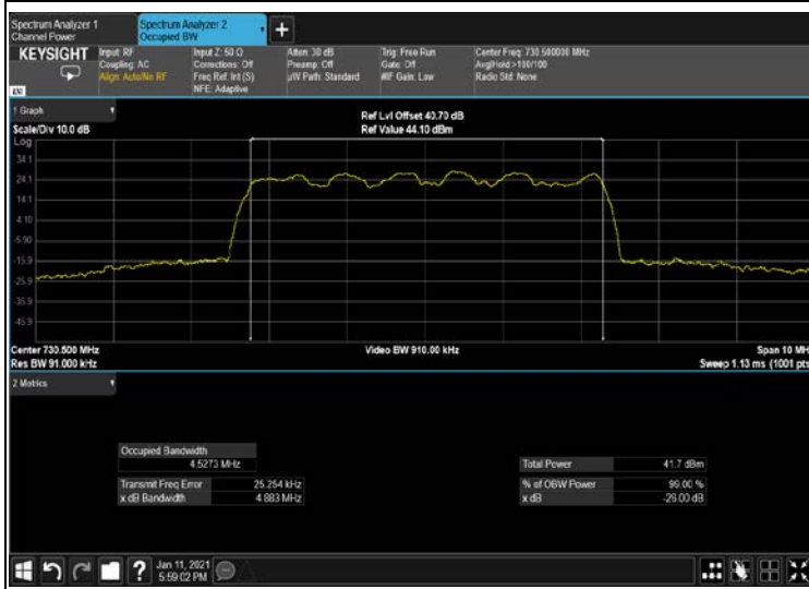
Figure 273: 16QAM 5MHz B.W; 730.5MHz, 15kHz OUTPUT
