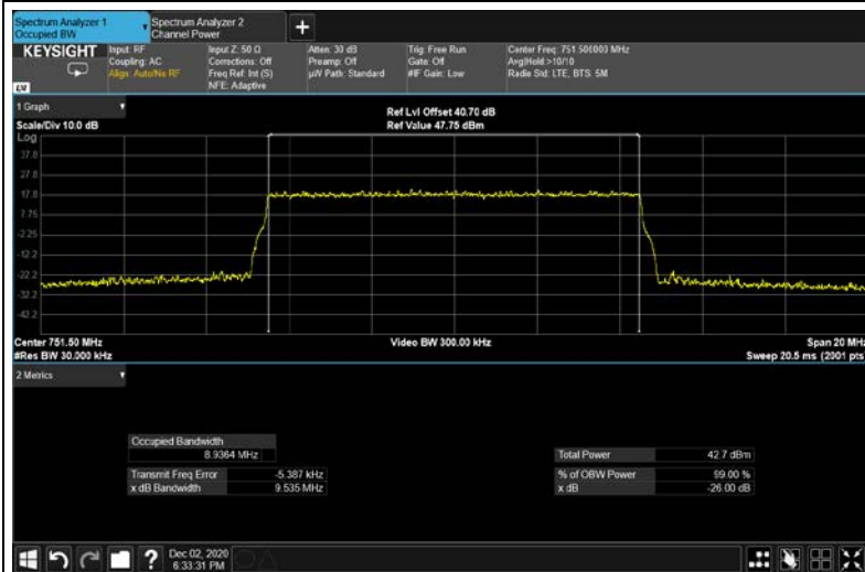
Figure 354: 16QAM 10MHz; 751.5MHz output 4G
