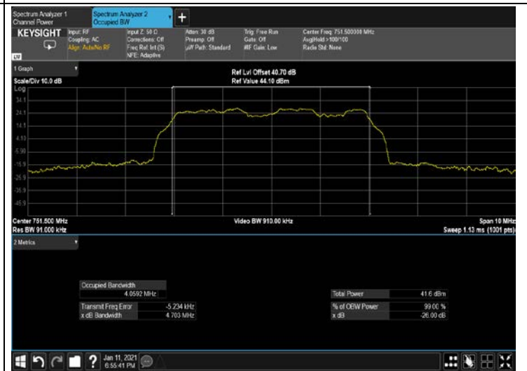
Figure 276: 16QAM 5MHz B.W; 751.5MHz, 30kHz OUTPUT
