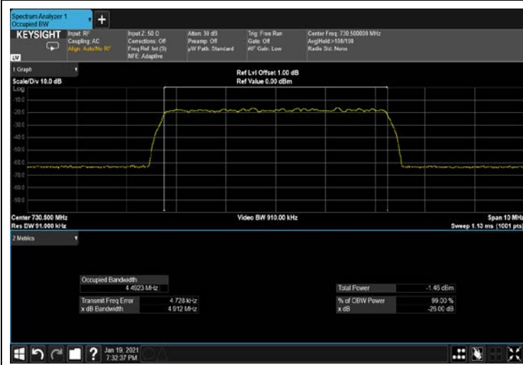
Figure 245: 256QAM 5MHz B.W; 730.5MHz, 15kHz INPUT
