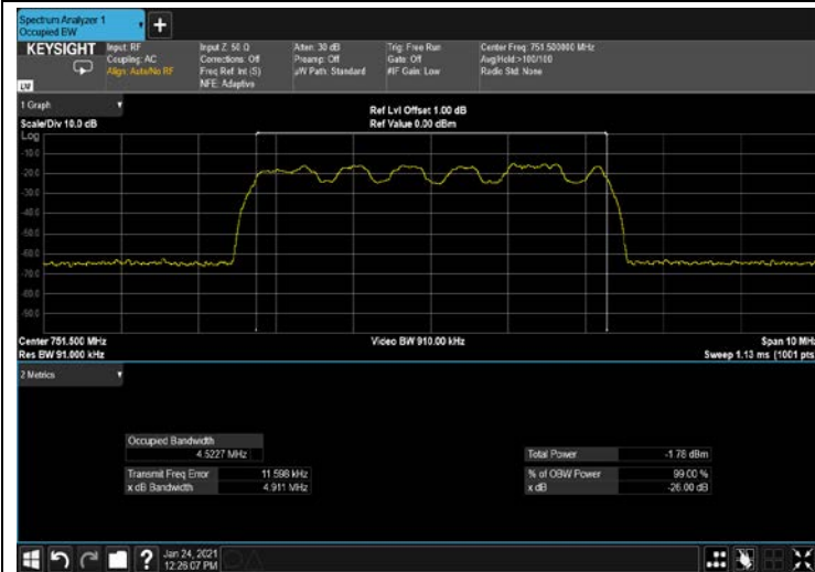
Figure 261: QPSK 5MHz B.W; 751.5MHz, 15kHz INPUT
