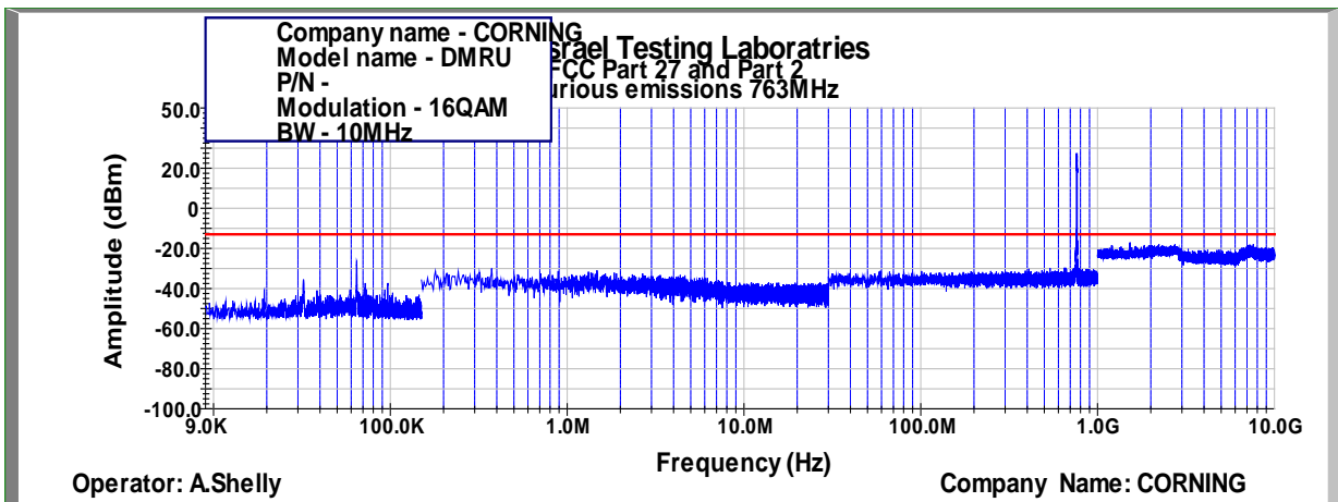
Figure 379: Spurious Emissions at Antenna Terminal 16QAM, 763MHz, B.W. 10MHz, Sub Carrier 15kHz
