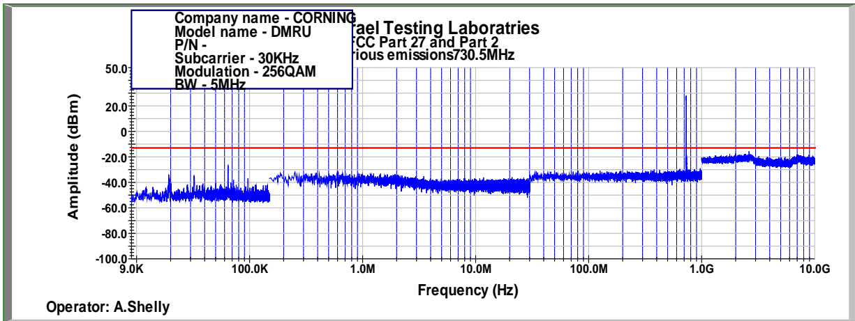
Figure 402: Spurious Emissions at Antenna Terminal 256QAM. 730.5MHz, B.W. 5MHz, Sub Carrier 30kHz
