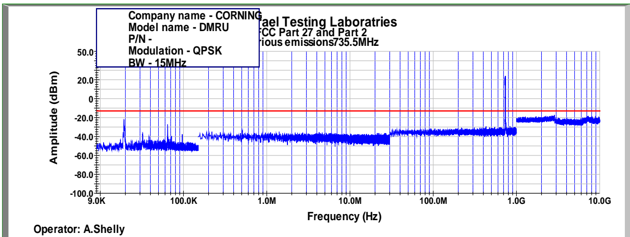
Figure 447: Spurious Emissions at Antenna Terminal QPSK, 735.5MHz, B.W. 15MHz
