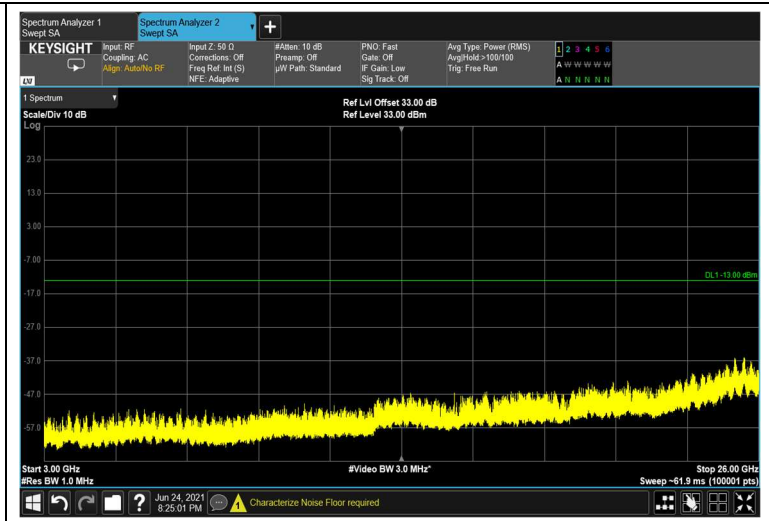
Spurious Emissions at Antenna Terminal 256QAM 60MHz B.W.; 2660.0MHz, 30kHz
