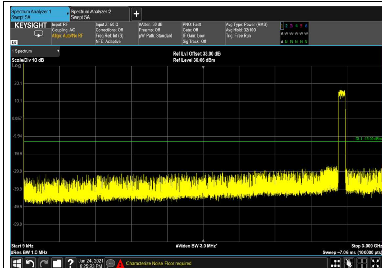
Spurious Emissions at Antenna Terminal 256QAM 60MHz B.W.; 2660.0MHz, 30kHz
