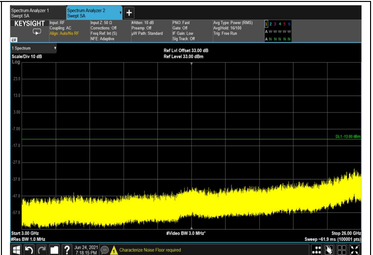
Spurious Emissions at Antenna Terminal 256QAM 60MHz B.W.; 2593.0MHz, 60kHz
