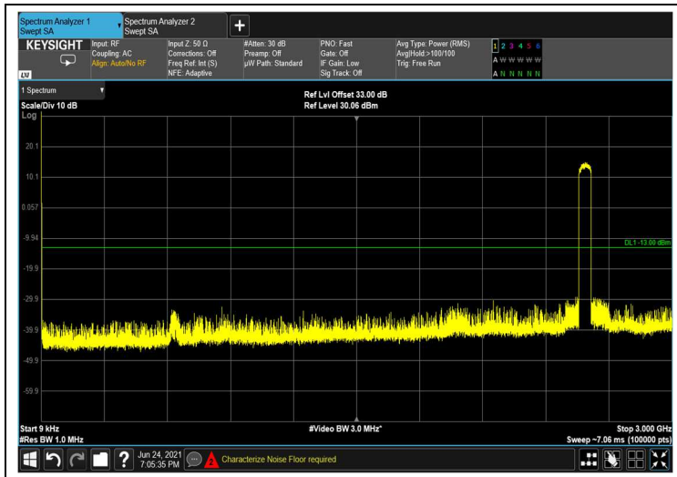
Spurious Emissions at Antenna Terminal 256QAM 60MHz B.W.; 2526.0MHz, 60kHz
