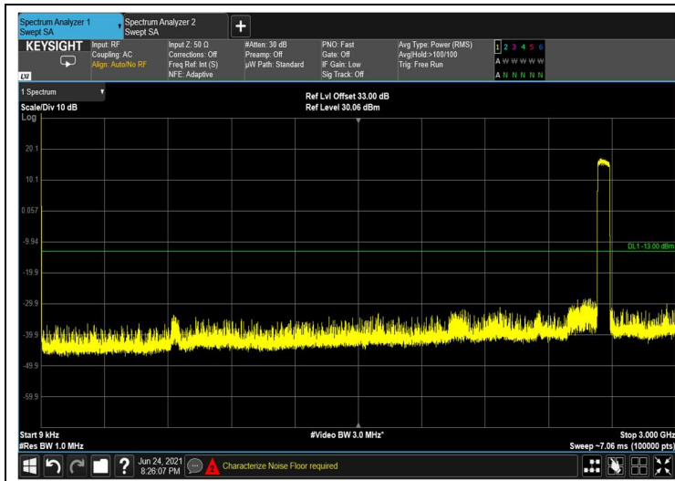
Spurious Emissions at Antenna Terminal 256QAM 60MHz B.W.; 2660.0MHz, 60kHz
