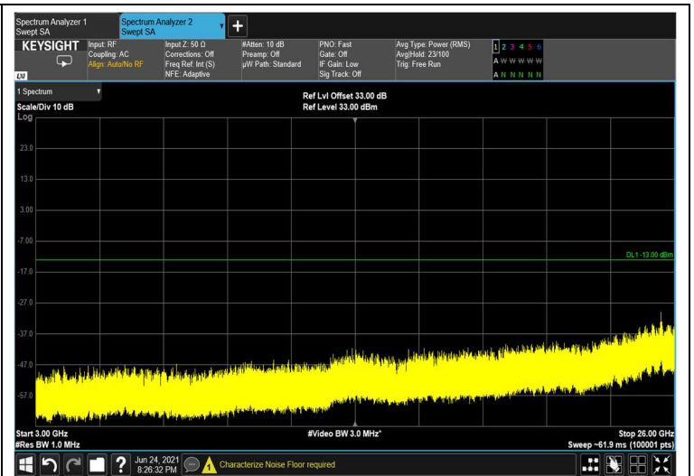
Spurious Emissions at Antenna Terminal 256QAM 60MHz B.W.; 2660.0MHz, 60kHz
