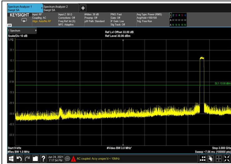
Spurious Emissions at Antenna Terminal 256QAM 60MHz B.W.; 2593.0MHz, 60kHz
