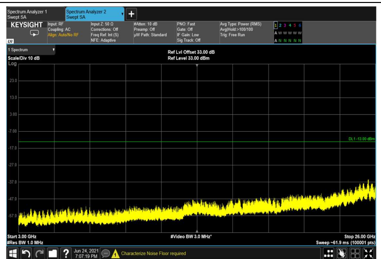
Spurious Emissions at Antenna Terminal 256QAM 60MHz B.W.; 2526.0MHz, 60kHz
