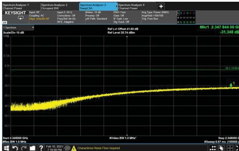
Figure 137. — 2345.0 MHz-2348.0MHz –QPSK,15KHz-5G
