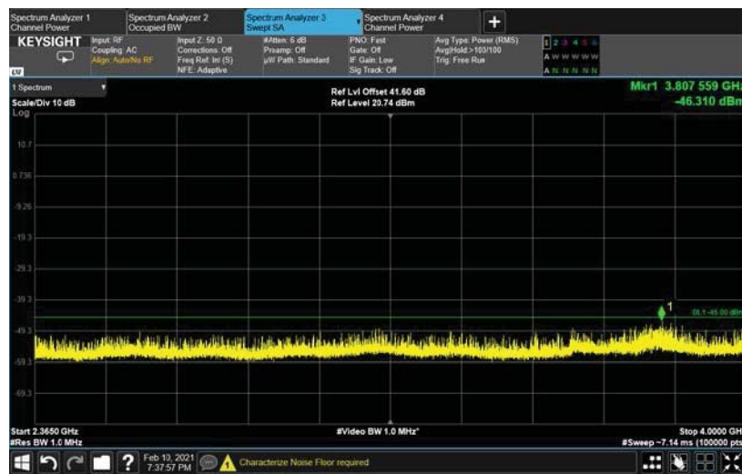
Figure 101. — 2365.0MHz-4000.0MHz -16QAM,30KHz-5G
