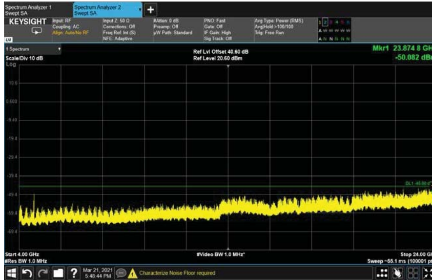
Figure 150. — 4000.0MHz-24000.0MHz –QPSK,30KHz-5G
