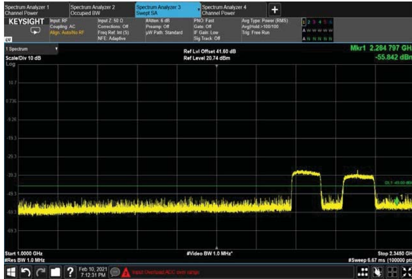
Figure 129. — 1000.0MHz-2345.0MHz –256QAM,30KHz-5G
