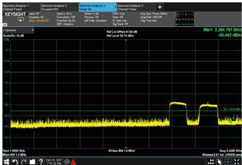
Figure 104. — 1000.0 MHz-2345.0MHz –64QAM,15KHz-5G
