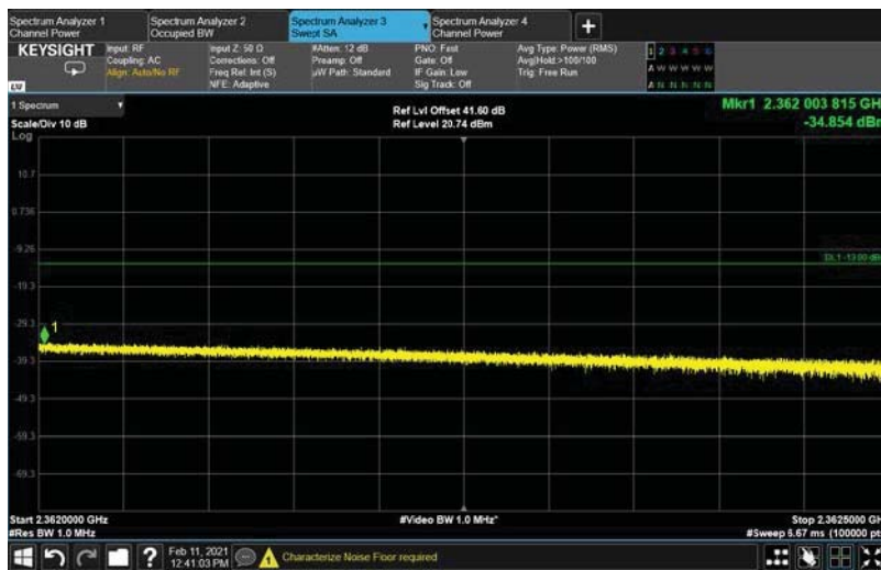
Figure 92. — 2362.0MHz-2362.5MHz –16QAM,15KHz-5G
