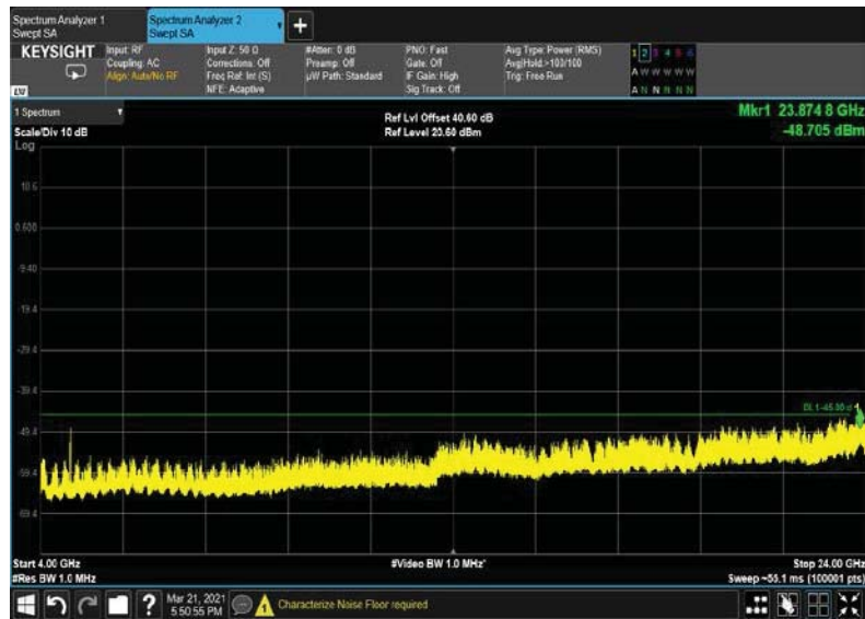
Figure 118. — 4000.0MHz-24000.0MHz -64QAM,30KHz-5G
