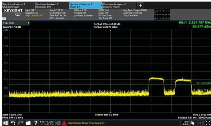
Figure 97. — 1000.0MHz-2345.0MHz -16QAM,30KHz-5G
