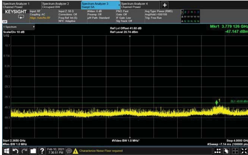
Figure 126. — 2365.0MHz-4000.0MHz –256QAM,15KHz-5G
