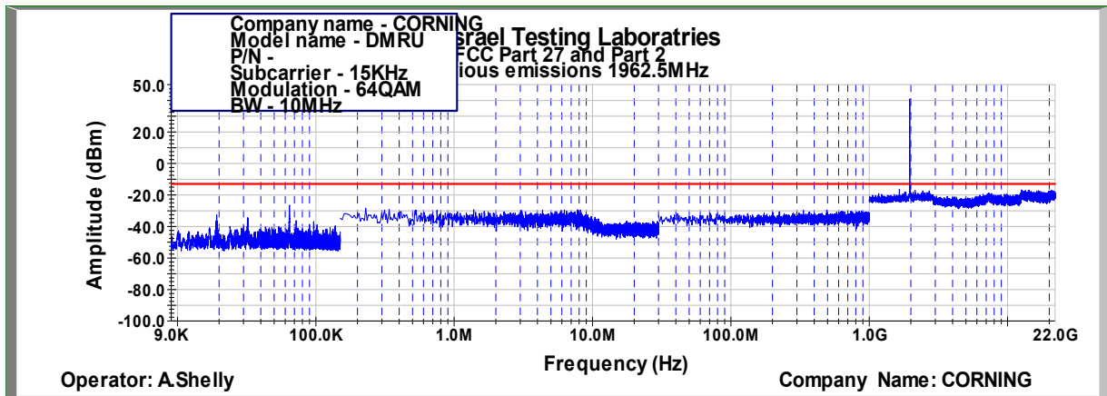
Figure 408: Spurious Emissions at Antenna Terminal 64QAM, 1962.5MHz, B.W. 10MHz, Sub Carrier 15kHz
