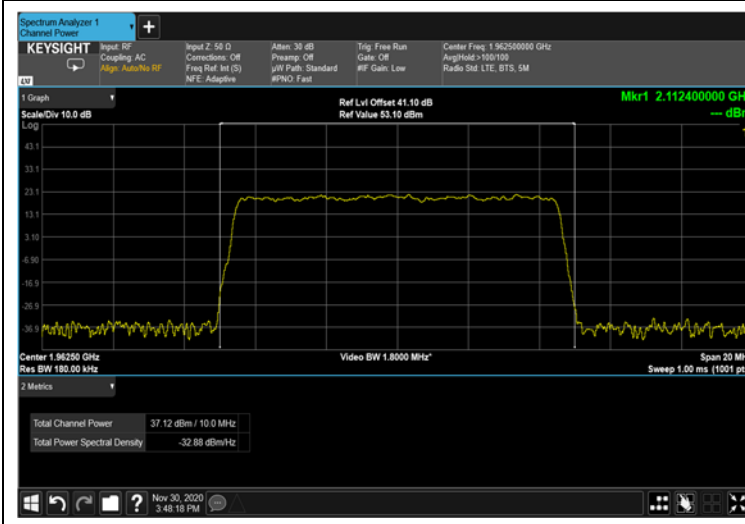
Figure 88: 16QAM 10MHz B.W.; 1962.5MHz – 4G
