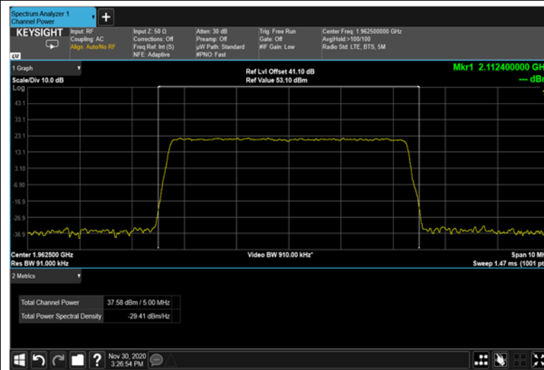
Figure 103: QPSK 5MHz B.W.; 1962.5MHz – 4G
