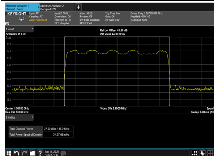
Figure 25: 16QAM 15MHz B.W.; 1987.5MHz, 15 kHz
