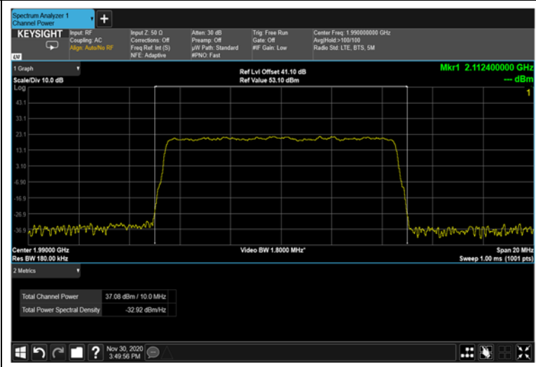
Figure 89: 16QAM 10MHz B.W.; 1990MHz – 4G
