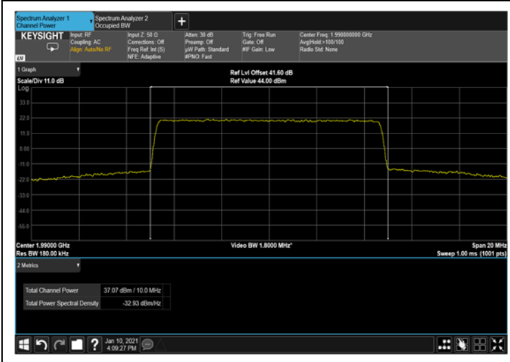
Figure 55: 256QAM 10MHz B.W.; 1990MHz, 15kHz
