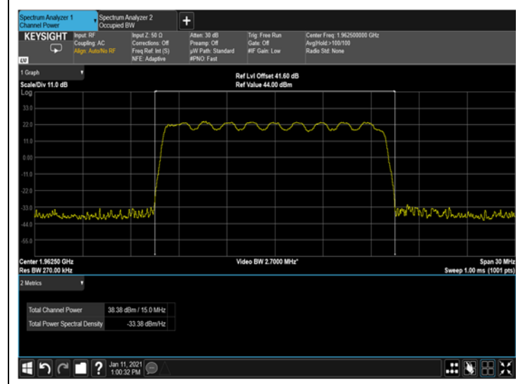
Figure 24: 16QAM 15MHz B.W.; 1962.5MHz, 30kHz
