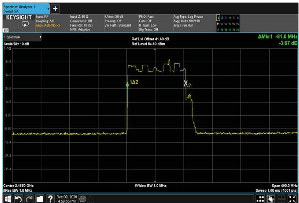
Figure 486. — Out-of-Band Rejection Plot
