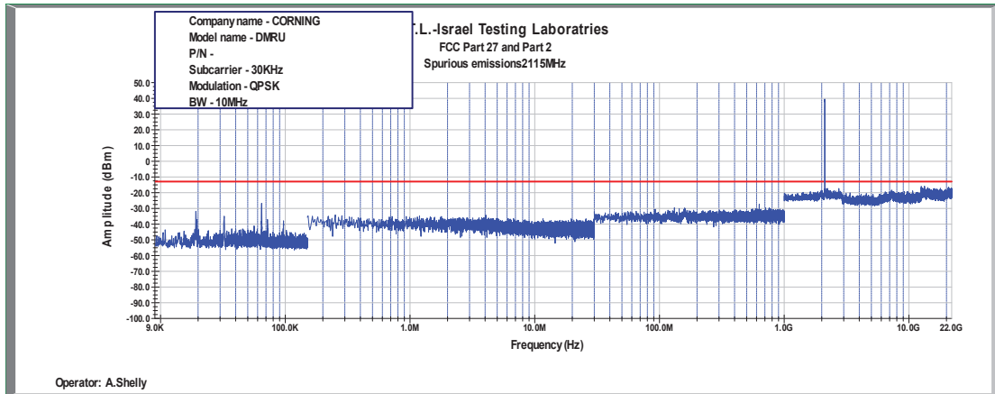
Figure 444: Spurious Emissions at Antenna Terminal QPSK, 2115MHz, B.W. 10MHz, Sub Carrier 30kHz
