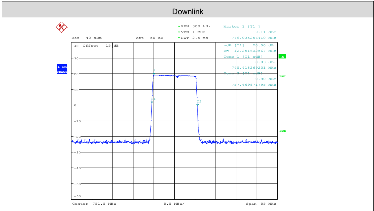
The peak of the frequency response f_0 is 746.04MHz
