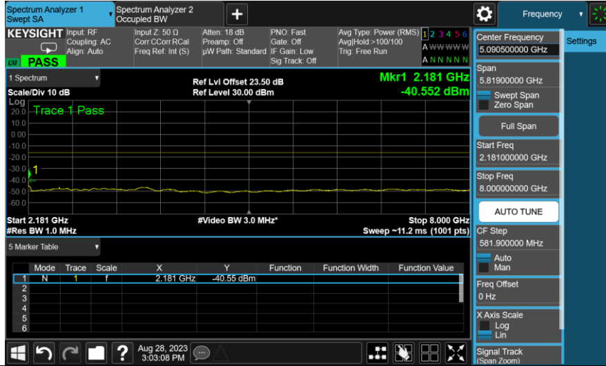
DL_1S_B_AWGN_Pre-AGC_Spurious emission 4
