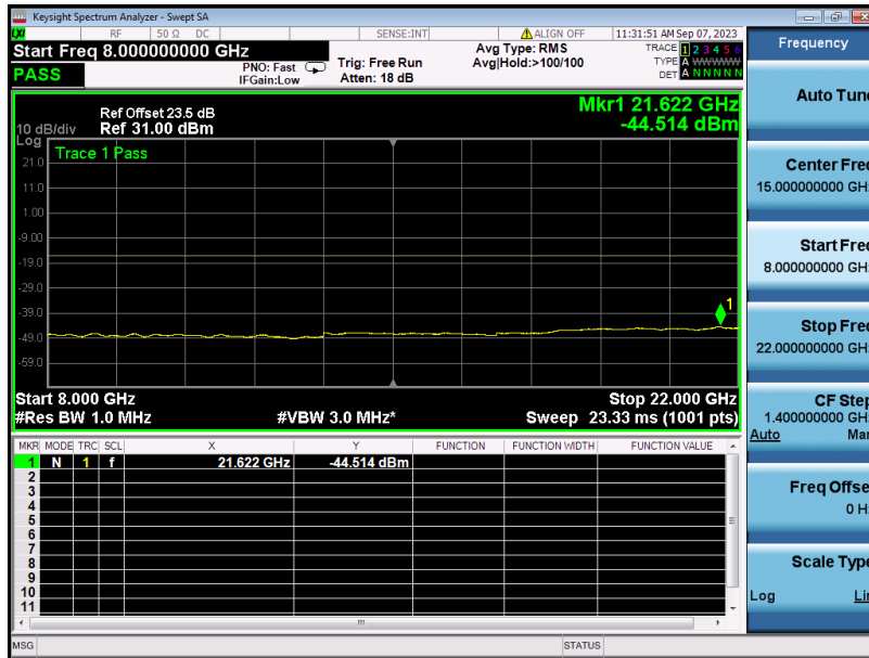
DL_1S_B_AWGN_Pre-AGC_Spurious emission 4
