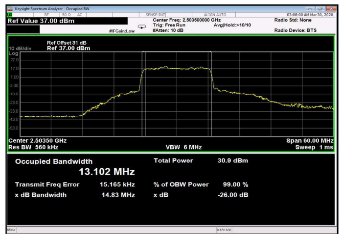
Figure 362: 64QAM 15MHz B.W.; 2503.5 MHz, 60kHz Output
