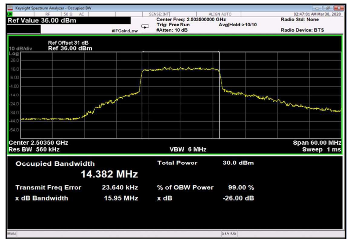
Figure 360: 64QAM 15MHz B.W.; 2503.5MHz, 15kHz Output
