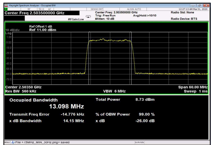
Figure 218: 64QAM 15MHz B.W.; 2503.5 MHz, 60kHz Input
