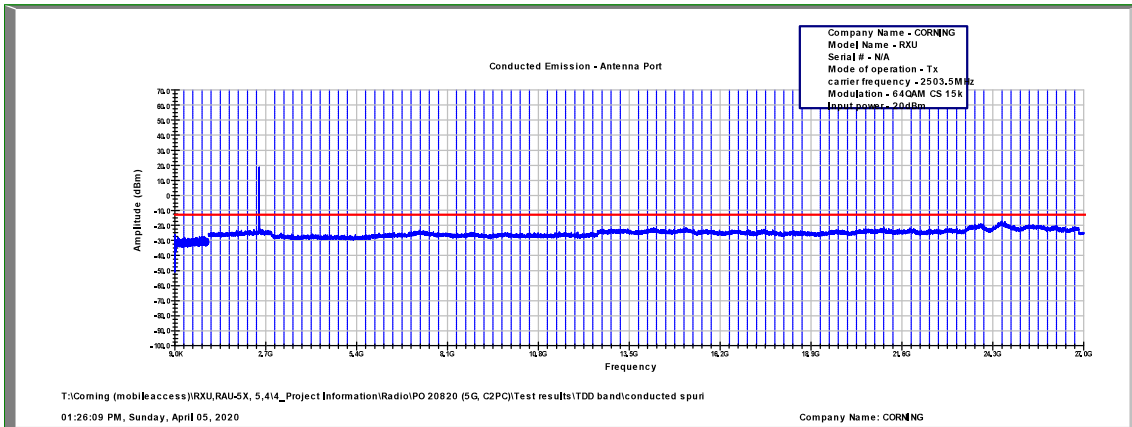
Figure 504: Spurious Emissions at Antenna Terminal 64QAM, 2503.5MHz, B.W. 15MHz, Sub Carrier 15kHz
