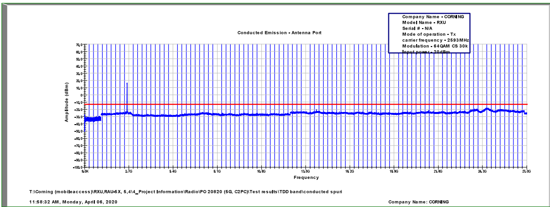
Figure 517: Spurious Emissions at Antenna Terminal 64QAM, 2593.0MHz, B.W. 20MHz, Sub Carrier 30kHz
