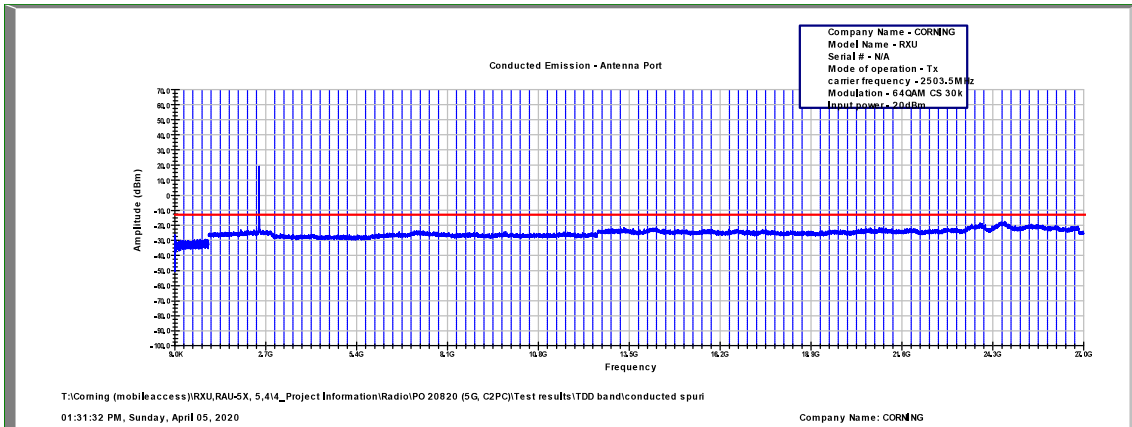
Figure 507: Spurious Emissions at Antenna Terminal 64QAM, 2503.5MHz, B.W. 15MHz, Sub Carrier 30kHz
