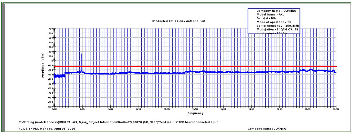
Figure 523: Spurious Emissions at Antenna Terminal 64QAM, 2593.0MHz, B.W. 40MHz, Sub Carrier 15kHz
