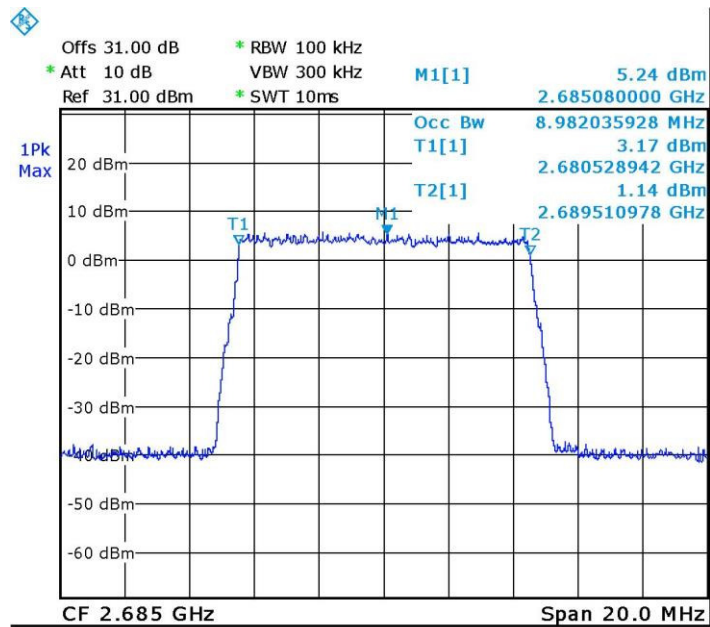
Figure 49 Occupied Bandwidth INPUT, 2685.0MHz, QPSK
