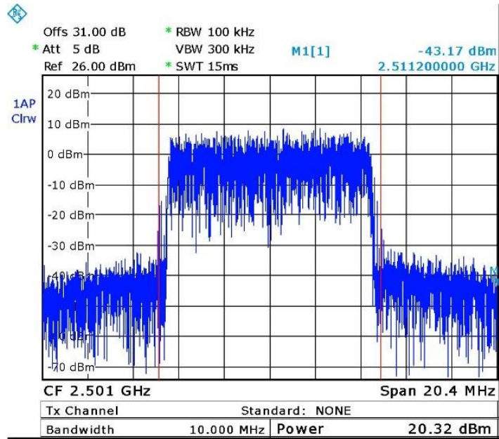
Figure 11. — 2501.0 MHz -64QAM
