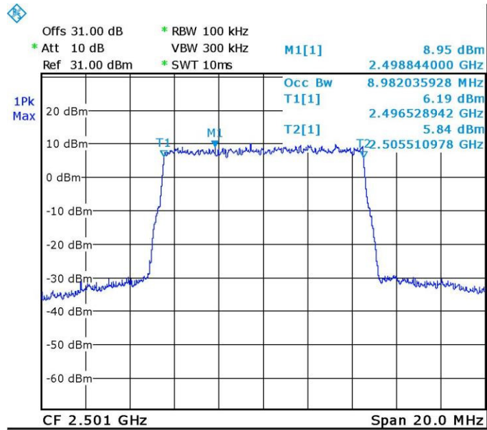
Figure 39 Occupied Bandwidth INPUT, 2501.0MHz, 16QAM
