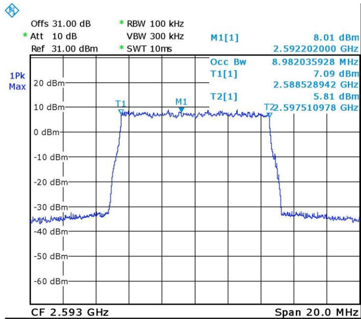
Figure 35 Occupied Bandwidth INPUT, 2593.0MHz, 64QAM
