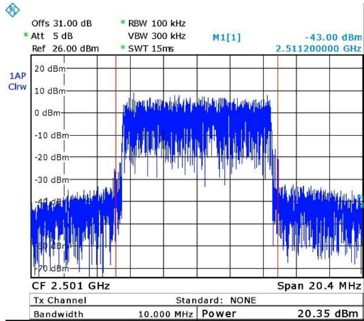
Figure 13. — 2501.0 MHz- QPSK
