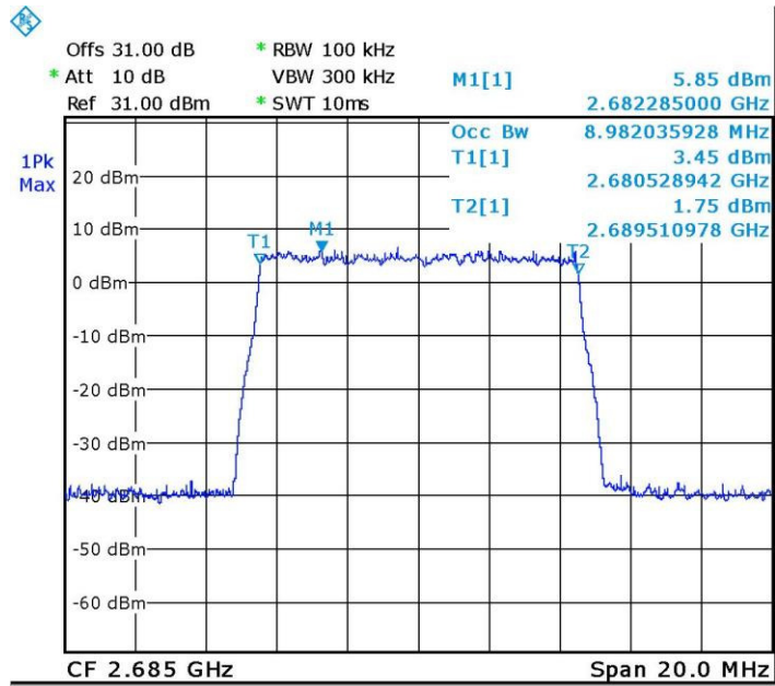
Figure 43 Occupied Bandwidth INPUT, 2685.0MHz, 16QAM
