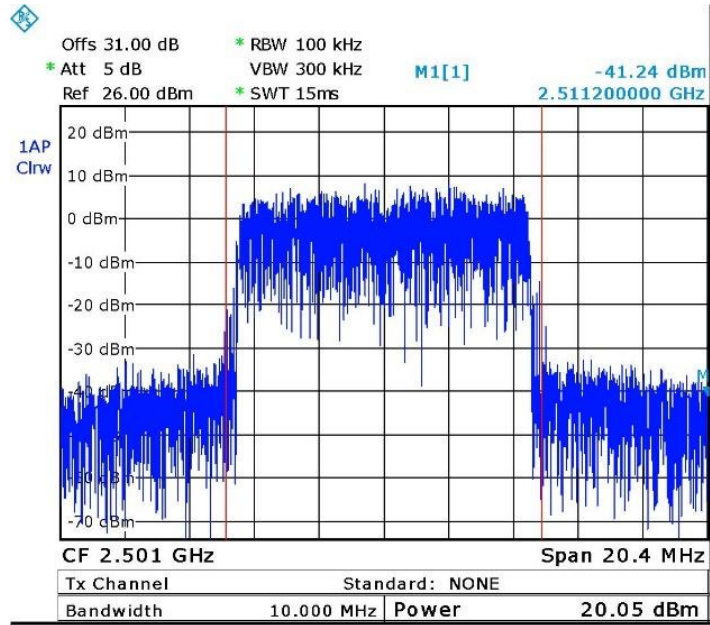
Figure 12. — 2501.0 MHz -16QAM
