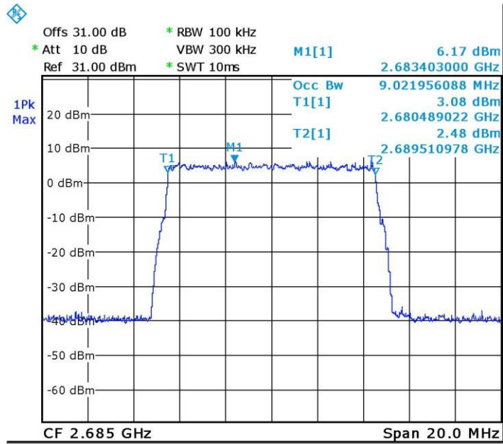
Figure 37 Occupied Bandwidth INPUT, 2685.0MHz, 64QAM
