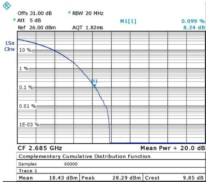
Figure 24. — 64QAM, 2685.0 MHz
