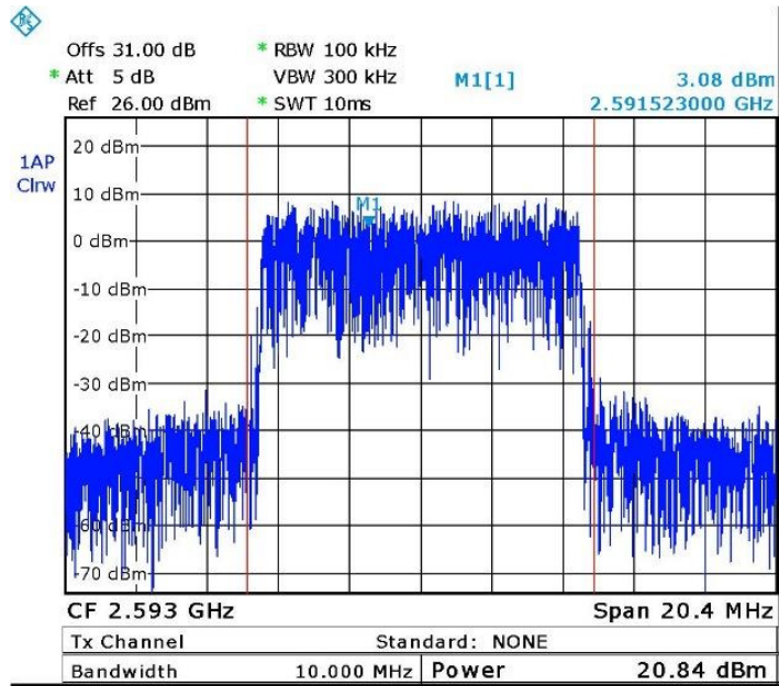
Figure 15. — 2593.0 MHz – 16QAM
