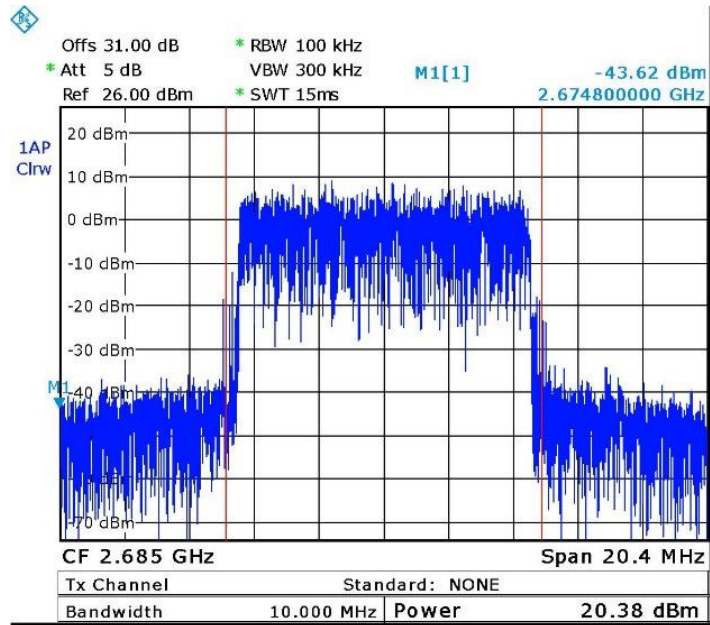
Figure 17. — 2685.0 MHz -64QAM
