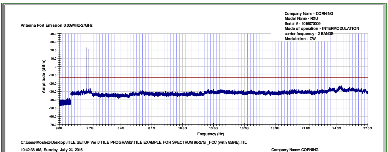
Figure 72 Intermodulation Conducted
