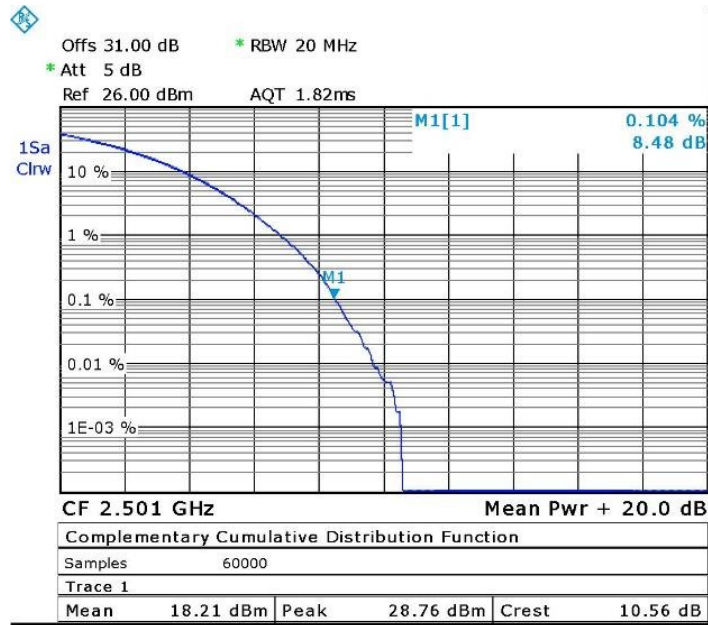
Figure 28. —QPSK, 2501.0 MHz
