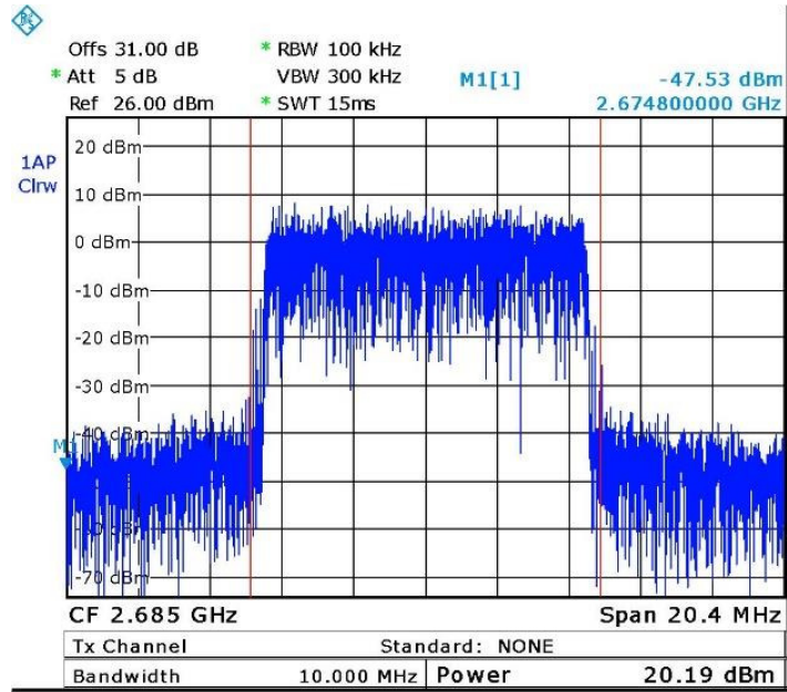
Figure 18. — 2685.0 MHz -16QAM
