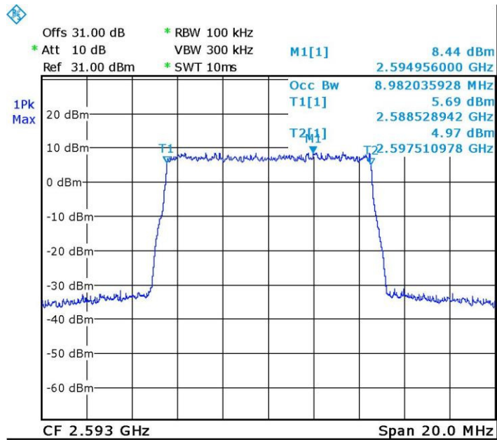
Figure 41 Occupied Bandwidth INPUT, 2593.0MHz, 16QAM
