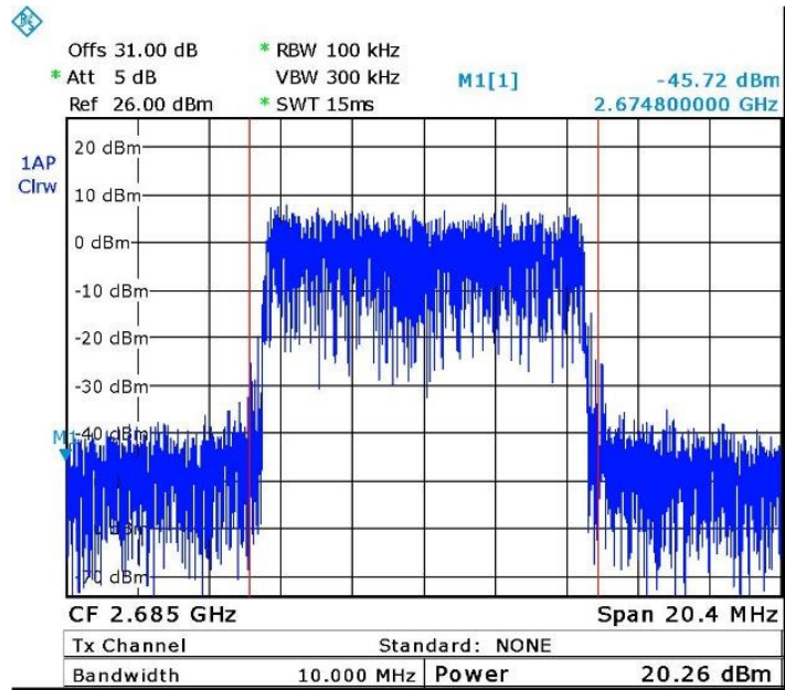
Figure 19. — 2685.0 MHz- QPSK
