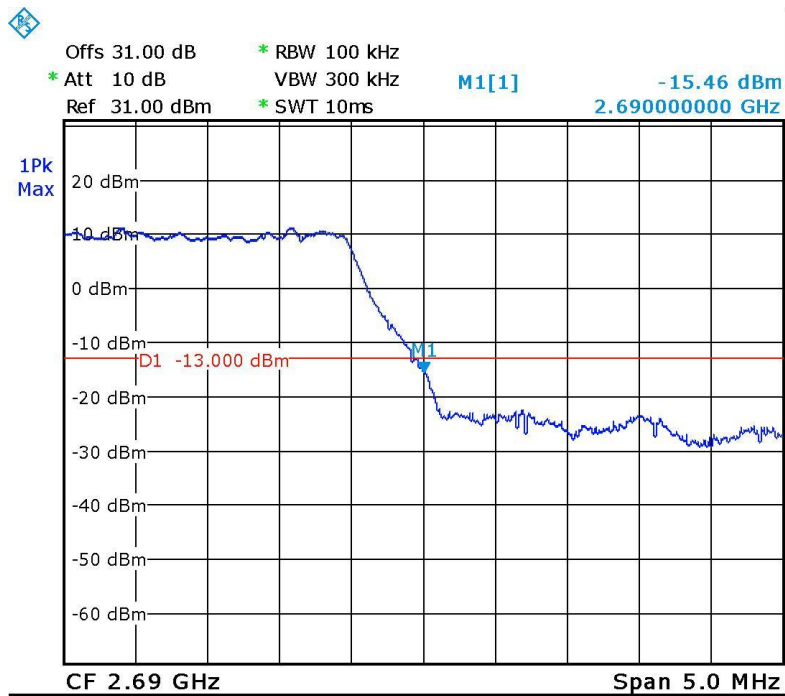
Figure 68. — Band Edge – High, QPSK
