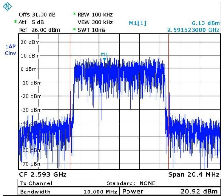
Figure 15. — 2593.0 MHz – 16QAM
