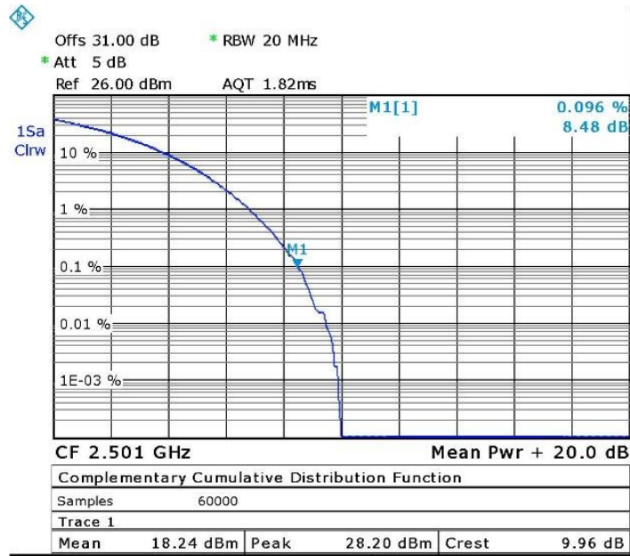
Figure 22. —64QAM, 2501.0 MHz
