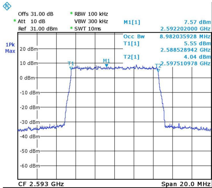
Figure 47 Occupied Bandwidth INPUT, 2593.0MHz, QPSK
