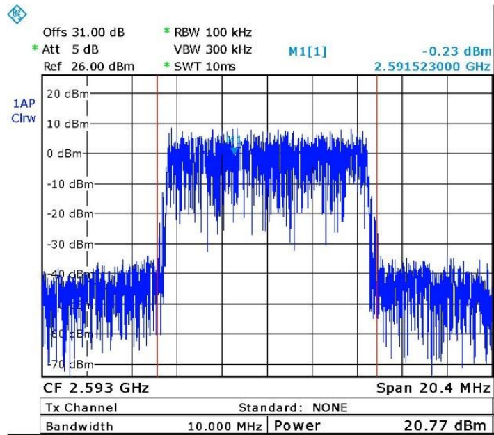
Figure 14. — 2593.0 MHz -64QAM
