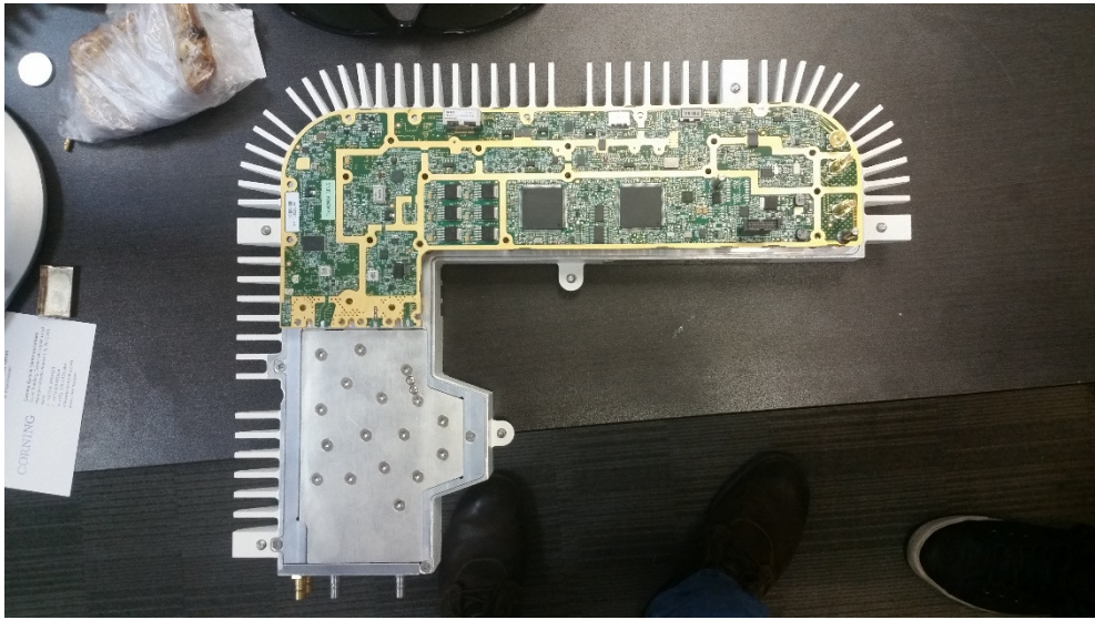
RF cavity filter with cover removed that is connected to end of PCB
