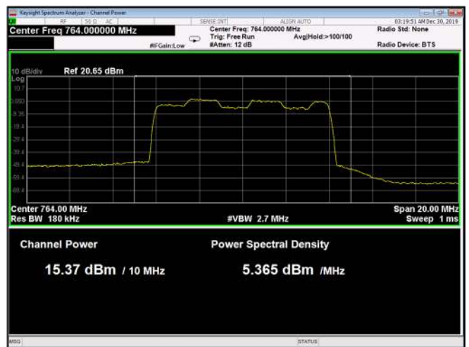
Figure 38: 64QAM 10MHz B.W.; 764.0 MHz, 60kHz
