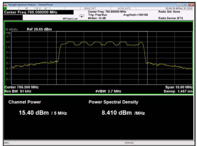
Figure 24: 64QAM 5MHz B.W.; 760.5MHz, 15kHz
