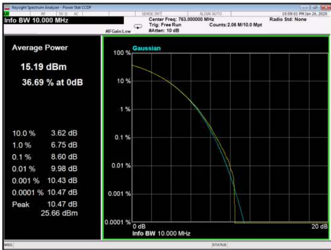
Figure 73: 16QAM 10MHz B.W.; 763.0MHz, 15kHz
