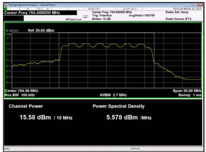
Figure 36: 64QAM 10MHz B.W.; 764.0MHz, 15kHz
