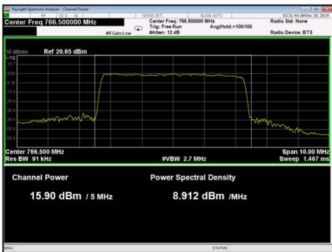
Figure 13: 16QAM 5MHz B.W.; 766.5MHz, 15kHz
