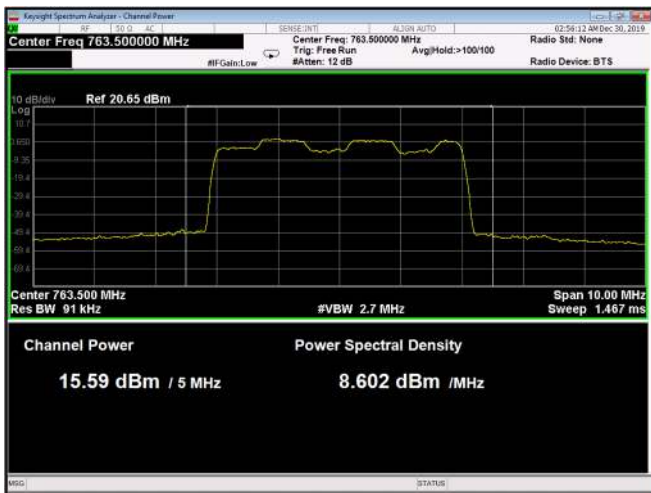
Figure 27: 64QAM 5MHz B.W.; 763.5MHz, 30kHz
