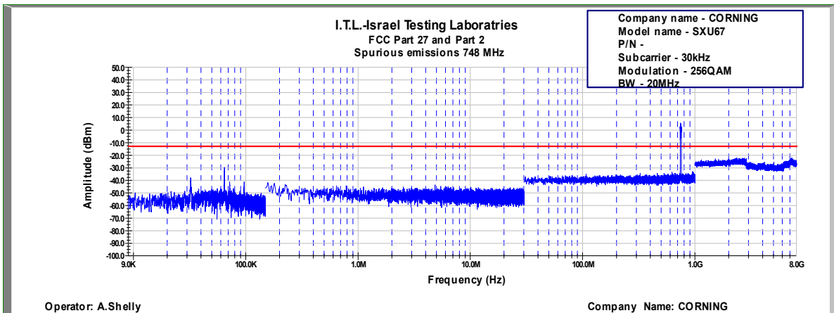
Figure 716: Spurious Emissions at Antenna Terminal 256QAM, 748.0MHz, B.W. 20MHz, Sub Carrier 30kHz
