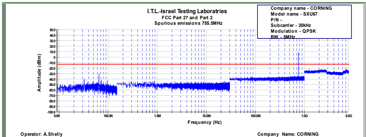
Figure 725: Spurious Emissions at Antenna Terminal QPSK, 755.5MHz, B.W. 5MHz, Sub Carrier 30kHz
