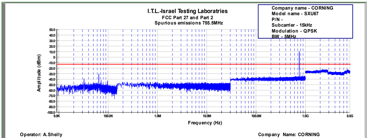
Figure 722: Spurious Emissions at Antenna Terminal QPSK, 755.5MHz, B.W. 5MHz, Sub Carrier 15kHz
