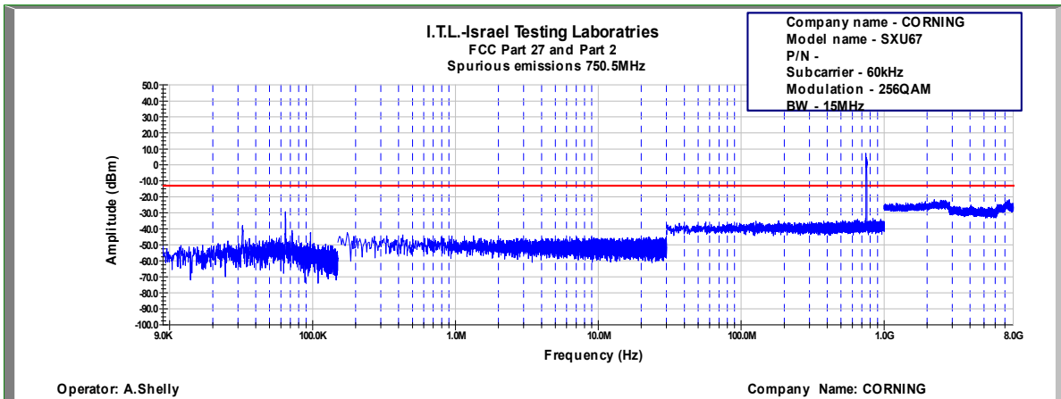
Figure 710: Spurious Emissions at Antenna Terminal 256QAM, 750.5MHz, B.W. 15MHz, Sub Carrier 60kHz
