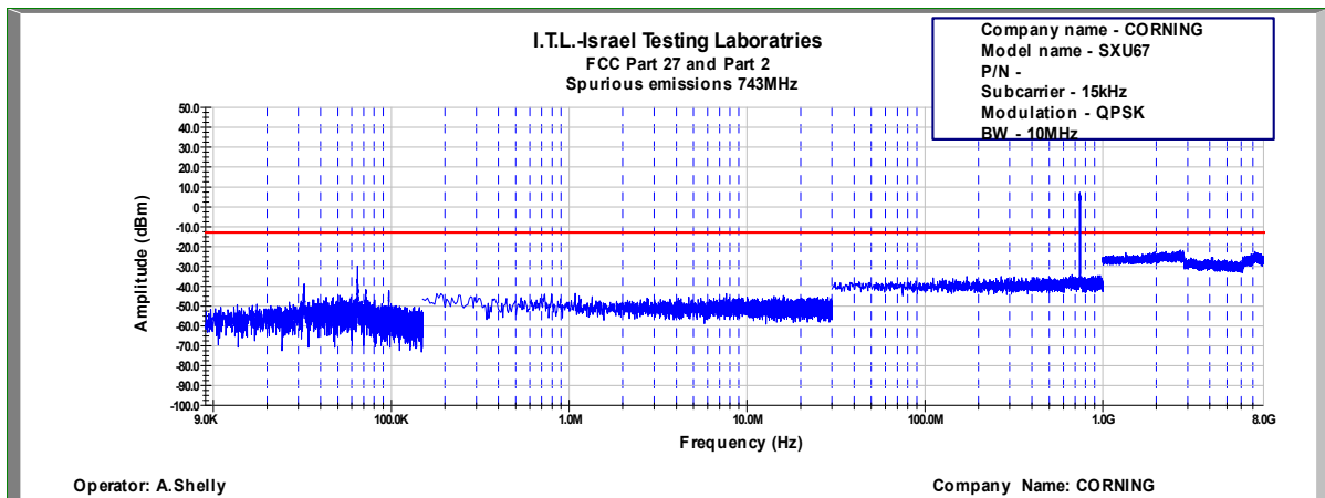
Figure 727: Spurious Emissions at Antenna Terminal QPSK, 743.0MHz, B.W. 10MHz, Sub Carrier 15kHz
