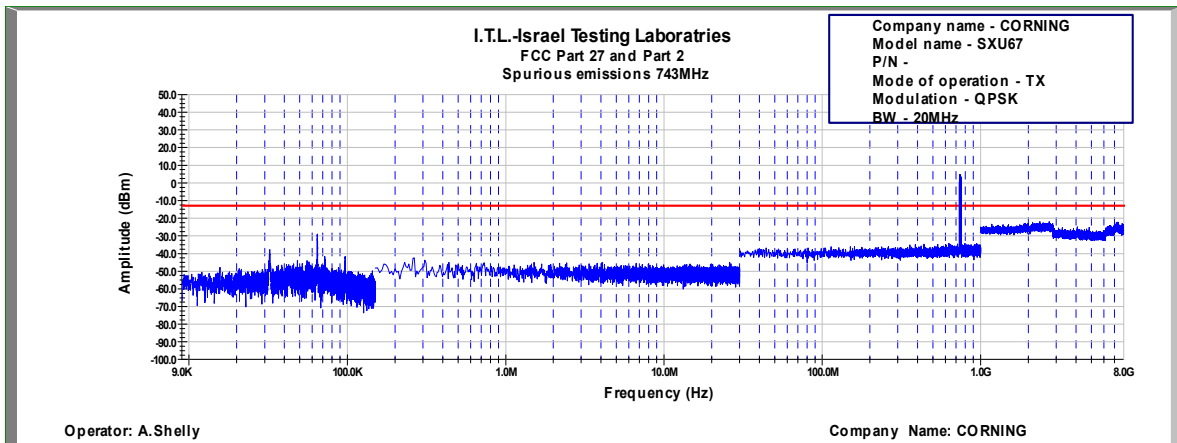
Figure 745: Spurious Emissions at Antenna Terminal QPSK, 743.0MHz, B.W. 20MHz, Sub Carrier 15kHz
