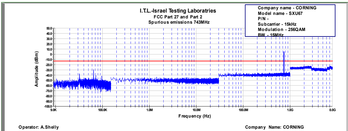
Figure 703: Spurious Emissions at Antenna Terminal 256QAM, 743.0MHz, B.W. 15MHz, Sub Carrier 15kHz
