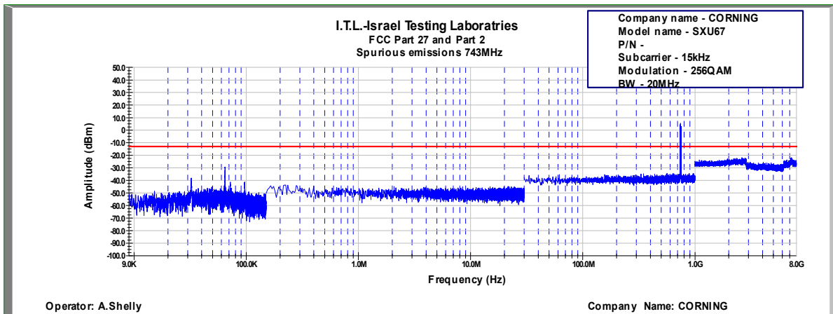
Figure 712: Spurious Emissions at Antenna Terminal 256QAM, 743.0MHz, B.W. 20MHz, Sub Carrier 15kHz
