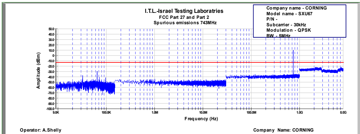
Figure 724: Spurious Emissions at Antenna Terminal QPSK, 743.0MHz, B.W. 5MHz, Sub Carrier 30kHz
