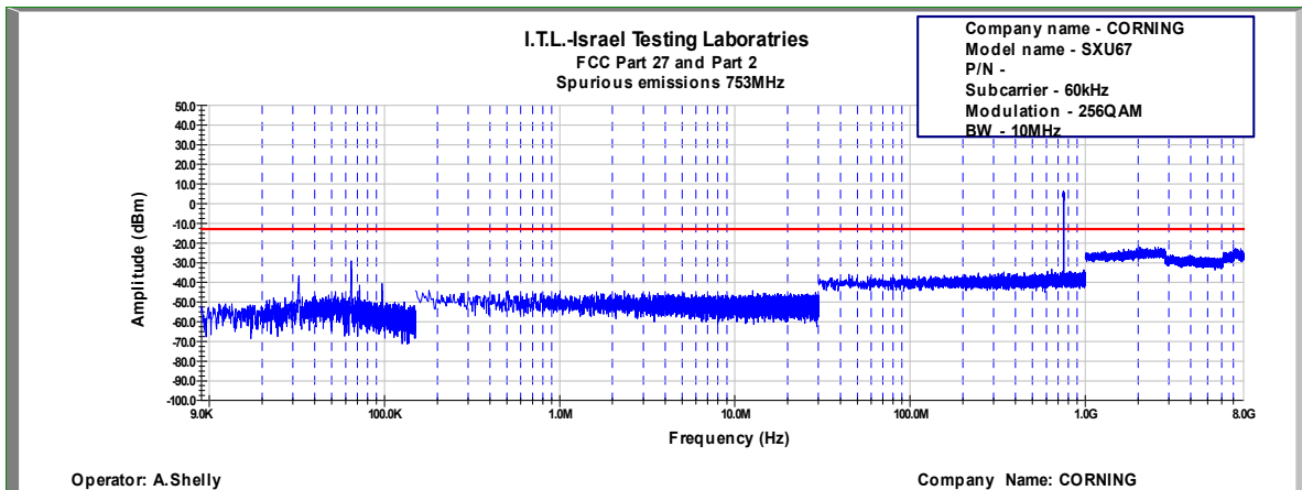
Figure 701: Spurious Emissions at Antenna Terminal 256QAM, 753.0MHz, B.W. 10MHz, Sub Carrier 60kHz
