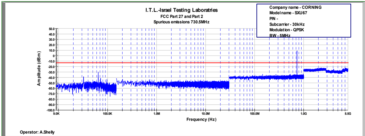
Figure 723: Spurious Emissions at Antenna Terminal QPSK, 730.5MHz, B.W. 5MHz, Sub Carrier 30kHz
