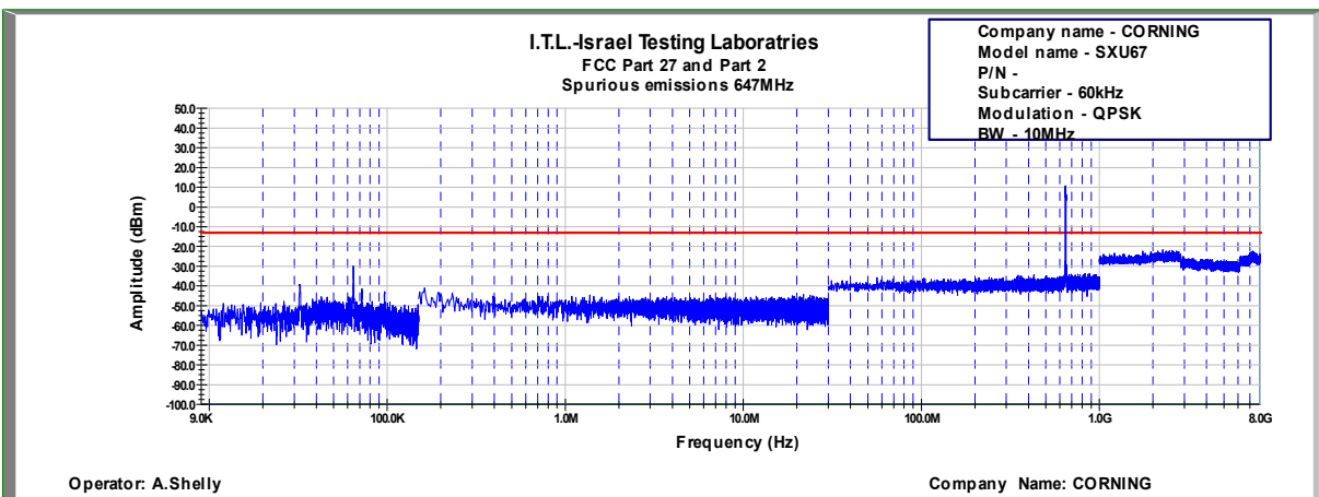
Figure 736: Spurious Emissions at Antenna Terminal QPSK, 647.0MHz, B.W. 10MHz, Sub Carrier 60kHz
