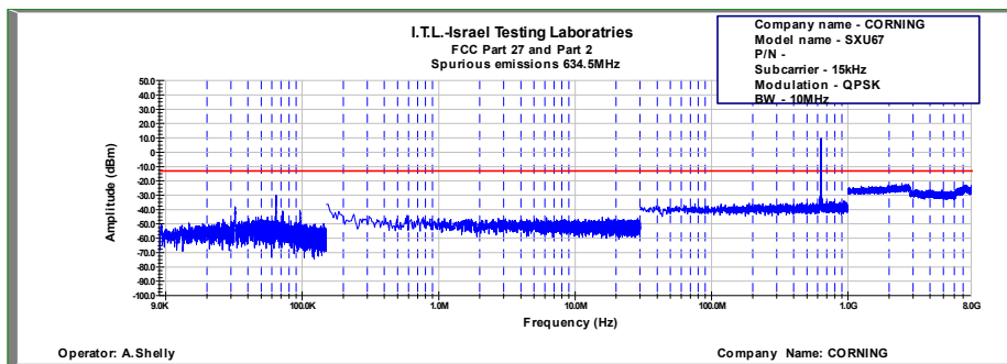
Figure 729: Spurious Emissions at Antenna Terminal QPSK, 634.5MHz, B.W. 10MHz, Sub Carrier 15kHz
