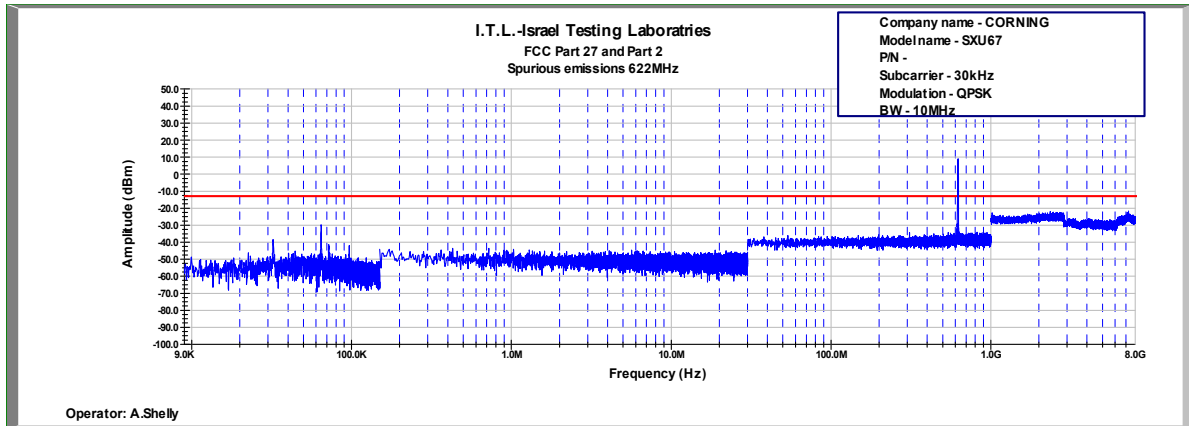
Figure 731: Spurious Emissions at Antenna Terminal QPSK, 622.0MHz, B.W. 10MHz, Sub Carrier 30kHz
