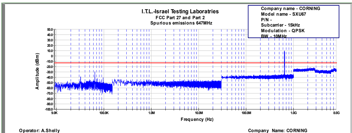
Figure 730: Spurious Emissions at Antenna Terminal QPSK, 647.0MHz, B.W. 10MHz, Sub Carrier 15kHz
