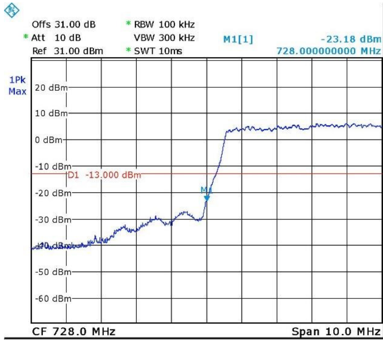
Figure 56. — QPSK 733.0 MHz
