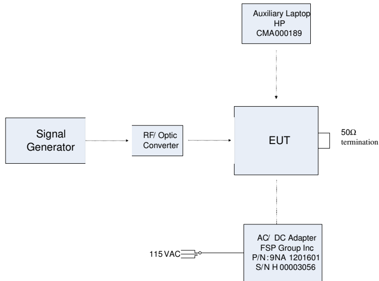
Figure 2. Radiated Test Set-Up
