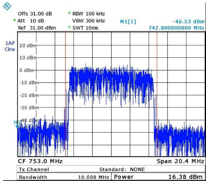
Figure 19. — QPSK 753 MHz
