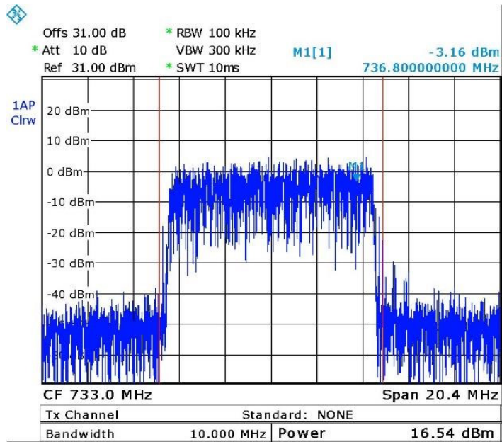
Figure 14. — 16QAM 733 MHz
