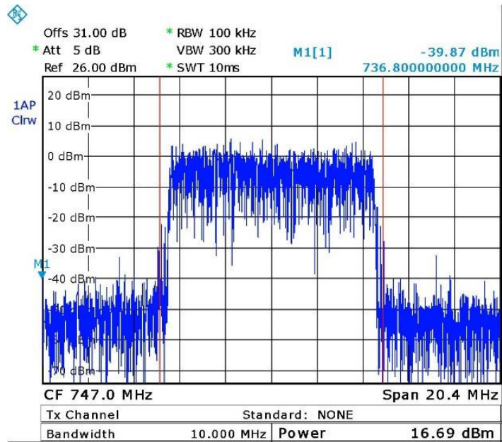
Figure 12. — 64QAM 747 MHz
