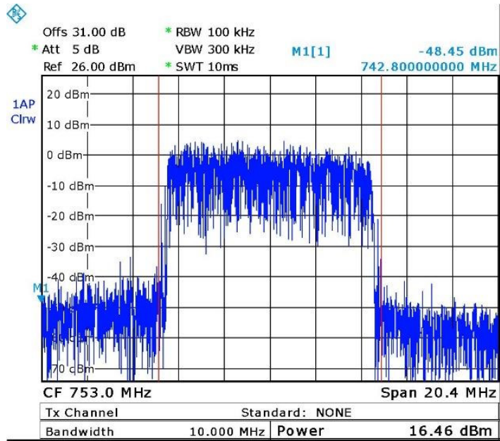
Figure 13. — 64QAM 753 MHz
