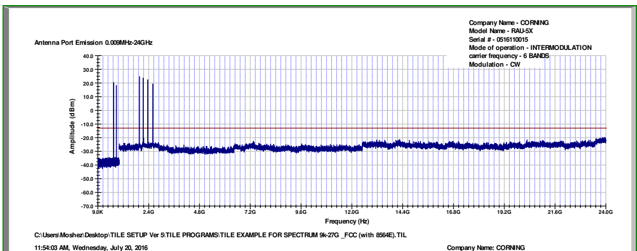
Figure 61 Intermodulation Conducted
