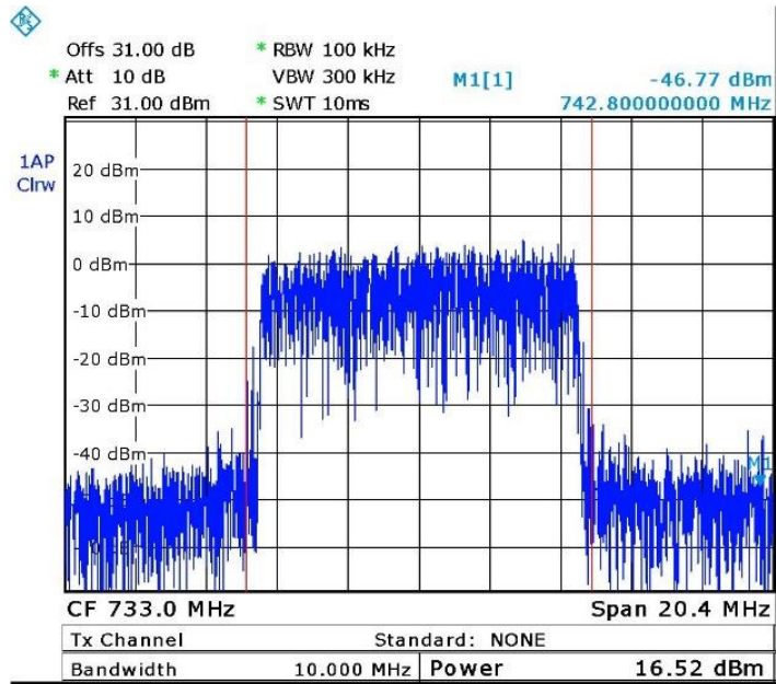
Figure 17. — QPSK 733 MHz
