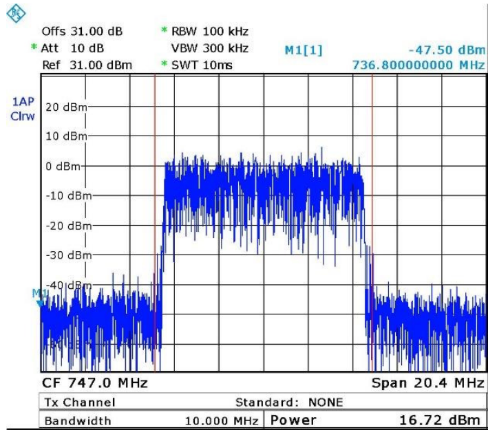
Figure 15. — 16QAM 747 MHz
