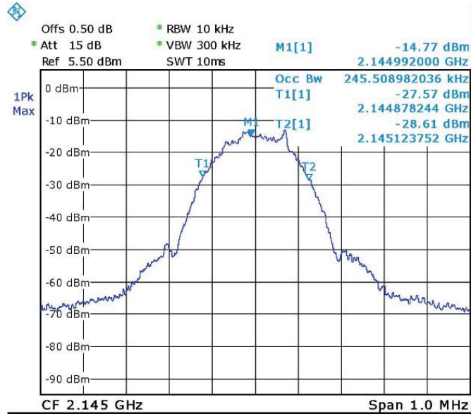
Figure 80. — GSM (2145.0 MHz) IN
