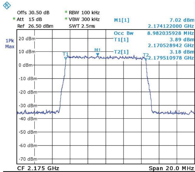
Figure 76. — LTE 64QAM (2175.0 MHz) IN
