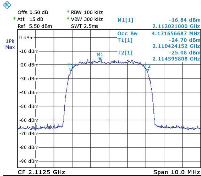
Figure 84. — WCDMA (2112.5 MHz) IN
