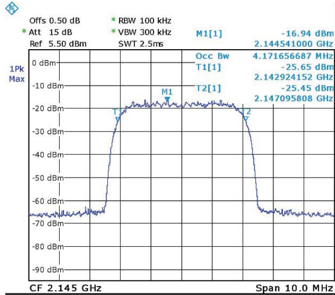
Figure 86. — WCDMA (2145.0 MHz) IN
