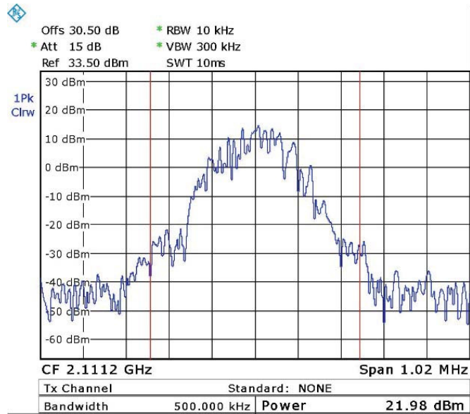
Figure 64. — GSM (2111.2 MHz)
