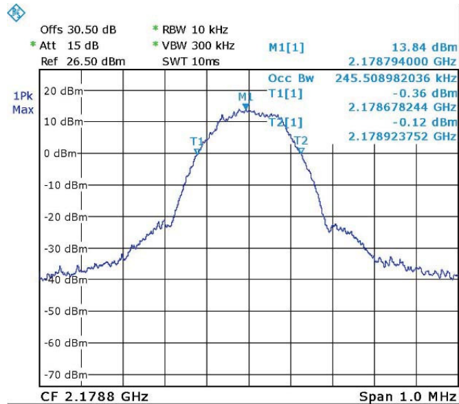
Figure 82. — GSM (2178.8 MHz) IN
