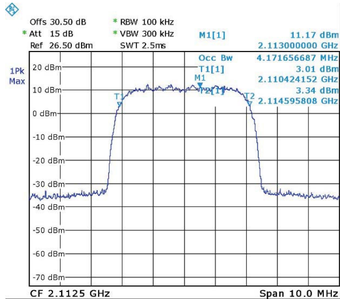
Figure 85. — WCDMA (2112.5 MHz) OUT
