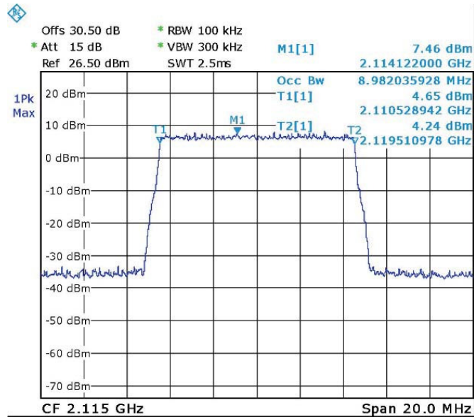
Figure 73. — LTE 64QAM (2115.0 MHz) OUT
