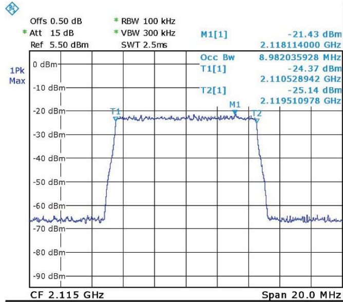
Figure 72. — LTE 64QAM(2115.0 MHz) IN
