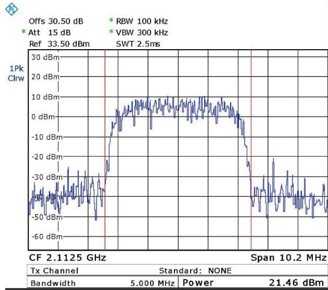
Figure 67. — WCDMA (2112.5 MHz)
