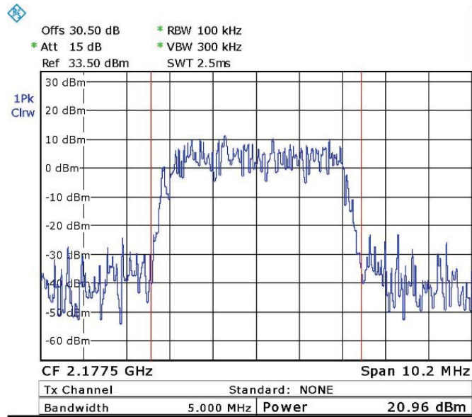
Figure 69. — WCDMA (2177.5 MHz)
