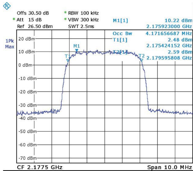
Figure 88. — WCDMA (2177.5 MHz) IN
