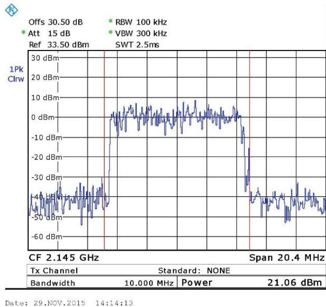
Figure 62. — LTE 64QAM (2145.0MHz)
