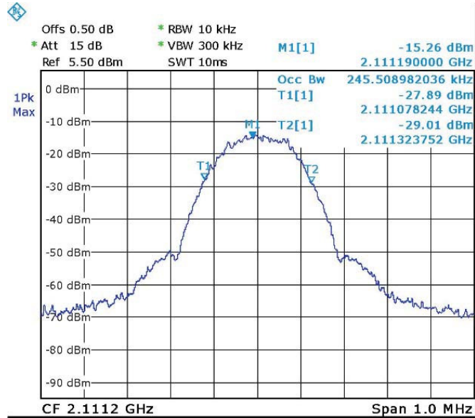
Figure 78. — GSM (2111.2 MHz) IN
