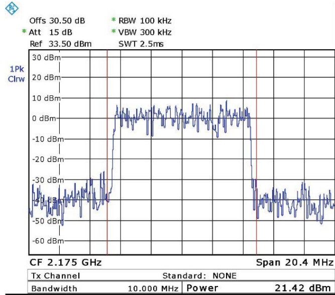
Figure 63. — LTE 64QAM (2175.0 MHz)
