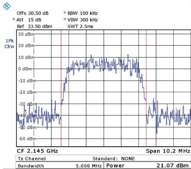
Figure 68. — WCDMA (2145.0 MHz)
