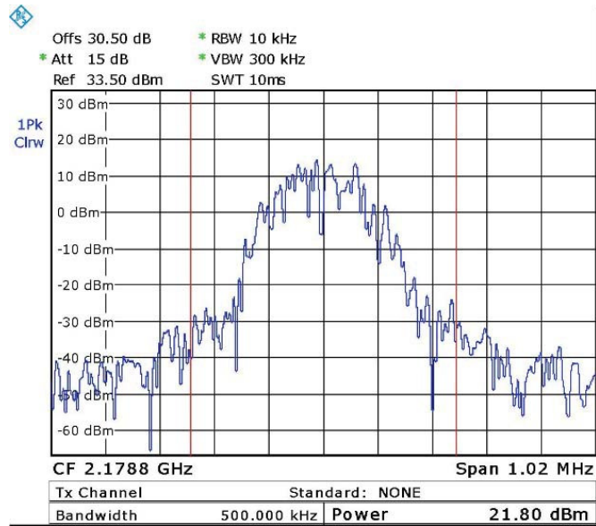
Figure 66. — GSM (2178.8 MHz)
