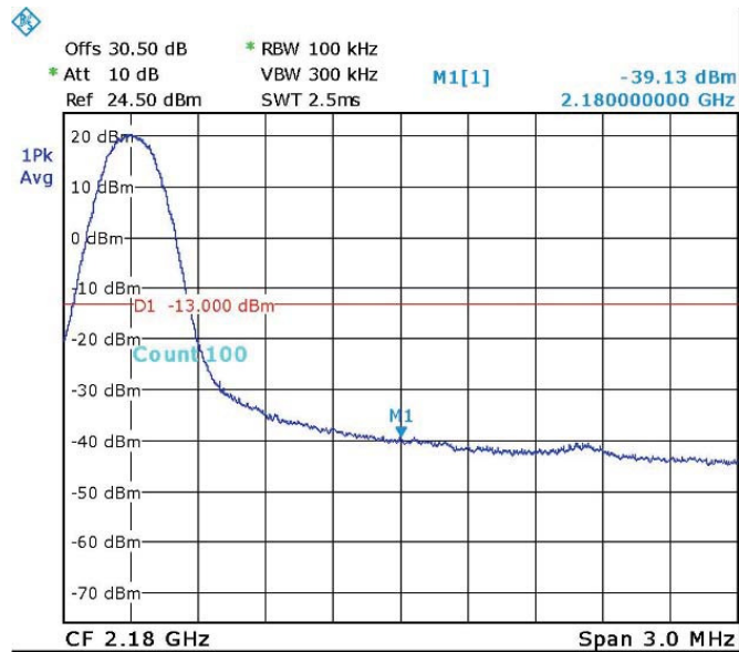
Figure 105. — GSM 2178.8 MHz
