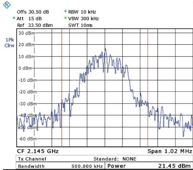
Figure 65. — GSM (2145.0 MHz)
