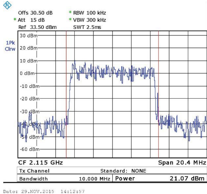
Figure 61. — LTE 64QAM (2115.0 MHz)
