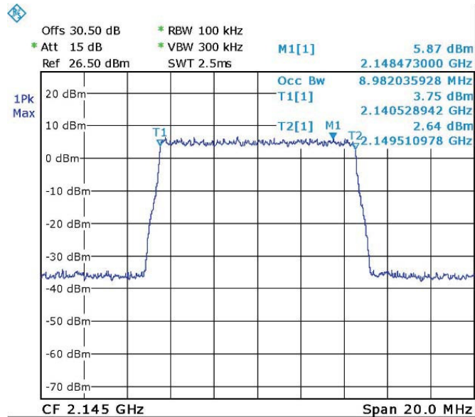
Figure 74. — LTE 64QAM (2145.0 MHz) IN
