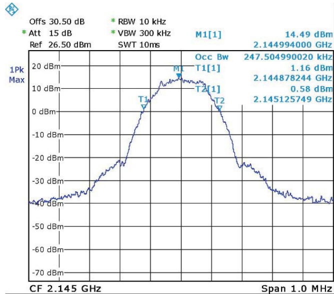
Figure 81. — GSM (2145.0 MHz) OUT
