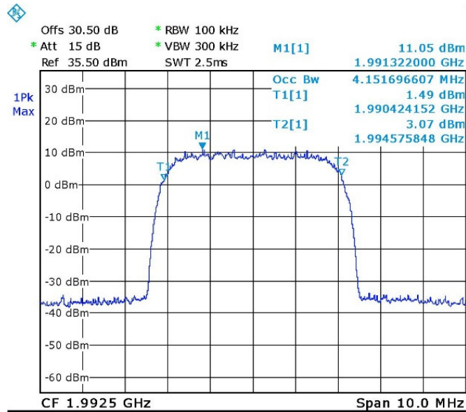
Figure 127. WCDMA - 1992.5 MHz Output
