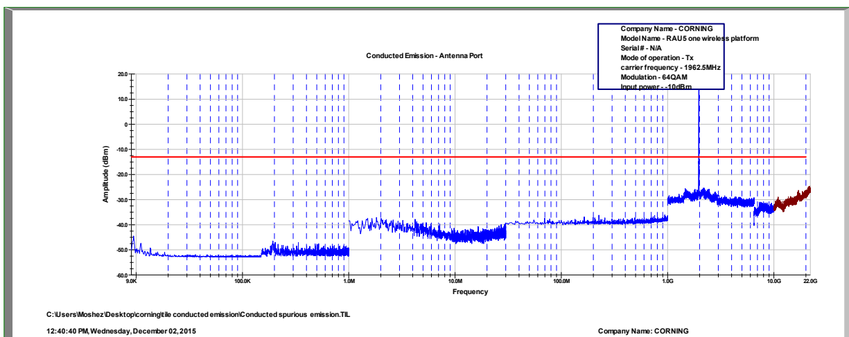
Figure 130 64QAM - 1962.5 MHz
