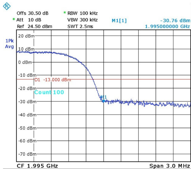
Figure 145—WCDMA - 1992.5 MHz
