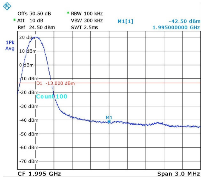
Figure 143— GSM - 1993.8 MHz
