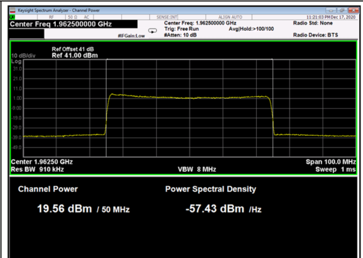
Figure 196: 256QAM 50MHz B.W.; 1962.5MHz, 30kHz
