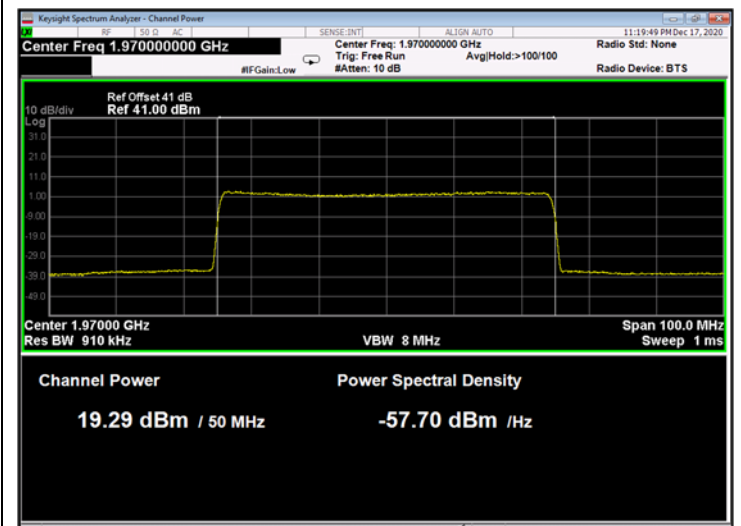
Figure 198: 256QAM 50MHz B.W.; 1970.0MHz, 15kHz
