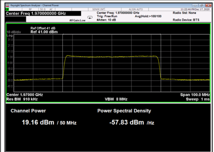
Figure 200: 256QAM 50MHz B.W.; 1970.0MHz, 60kHz
