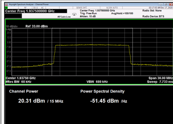
Figure 223: QPSK 15MHz B.W.; 1937.5MHz, 30kHz
