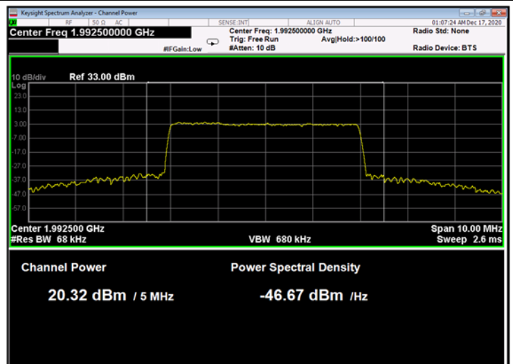
Figure 212: QPSK 5MHz C.S; 1992.5MHz, 30kHz
