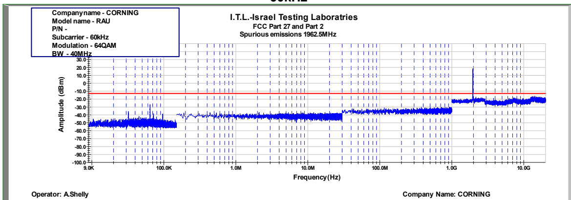
Figure 916: Spurious Emissions at Antenna Terminal 64QAM 40MHz B.W.; 1962.5MHz, 60kHz
