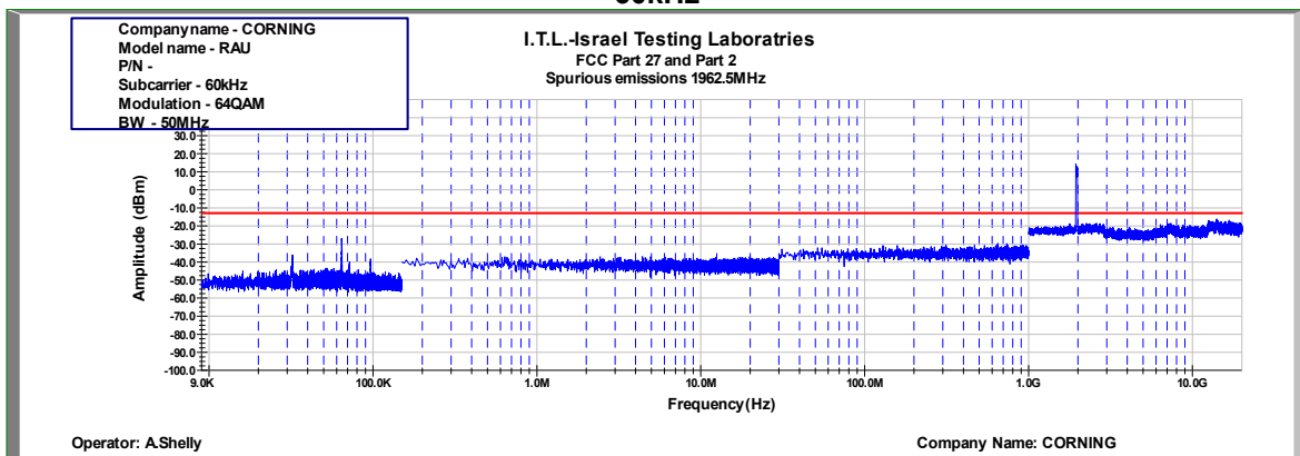
Figure 925: Spurious Emissions at Antenna Terminal 64QAM 50MHz B.W.; 1962.5MHz, 60kHz
