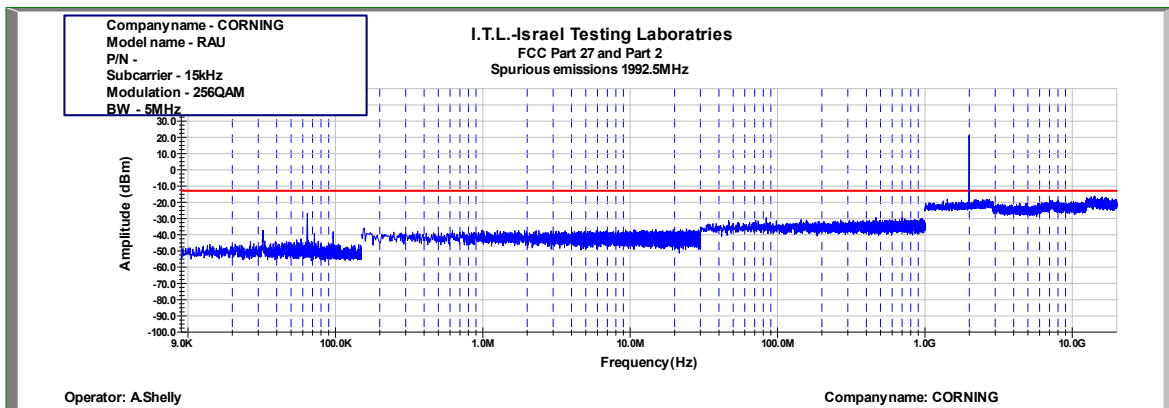
Figure 935: Spurious Emissions at Antenna Terminal 256QAM 5MHz B.W.; 1992.5MHz, 15kHz
