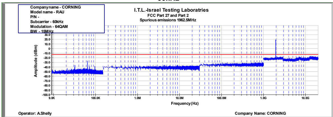
Figure 889: Spurious Emissions at Antenna Terminal 64QAM 15MHz B.W.; 1962.5MHz, 60kHz
