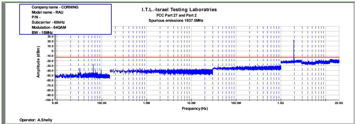
Figure 888: Spurious Emissions at Antenna Terminal 64QAM 15MHz B.W.; 1937.5MHz, 60kHz
