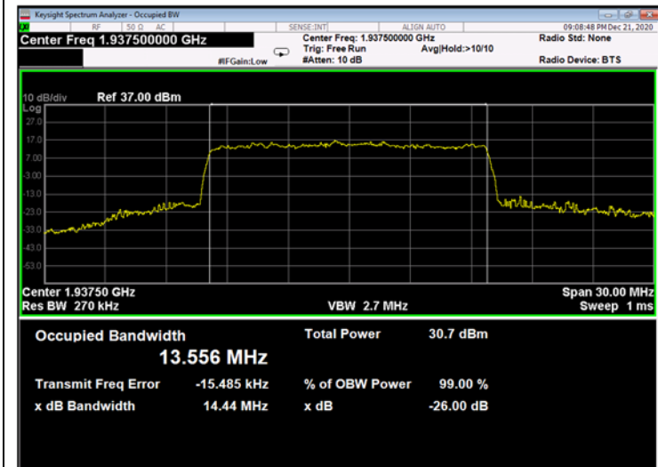
Figure 685: 256QAM 15MHz B.W.; 1937.5MHz, 30kHz - Output
