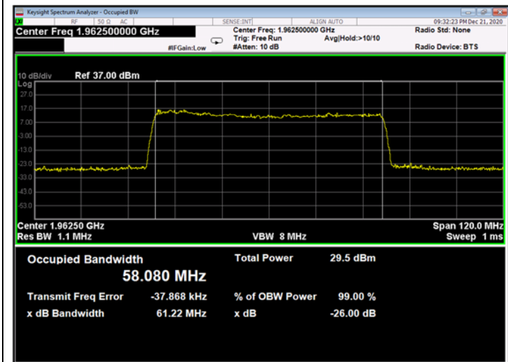
Figure 731: 256QAM 60MHz B.W.; 1962.5MHz, 30Hz - Output
