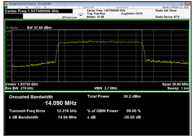
Figure 684: 256QAM 15MHz B.W.; 1937.5MHz, 15kHz - Output
