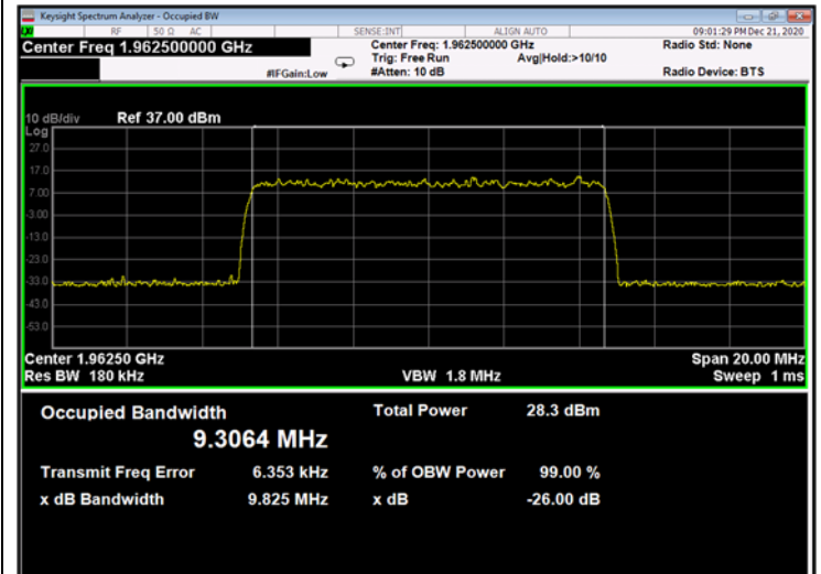
Figure 678: 256QAM 10MHz B.W.; 1962.5MHz, 15kHz - Output
