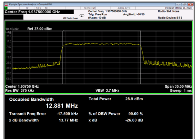
Figure 686: 256QAM 15MHz B.W.; 1937.5MHz, 60kHz - Output
