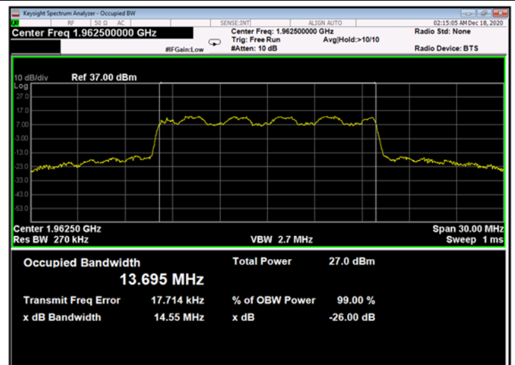
Figure 556: 16QAM 15MHz B.W.; 1962.5MHz, 30kHz - Output
