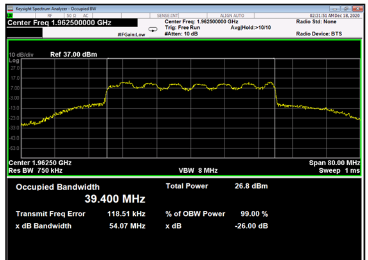
Figure 582: 16QAM 40MHz B.W.; 1962.5MHz, 15kHz - Output
