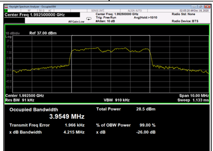
Figure 542: 16QAM 5MHz C.S; 1992.5MHz, 30kHz - Output
