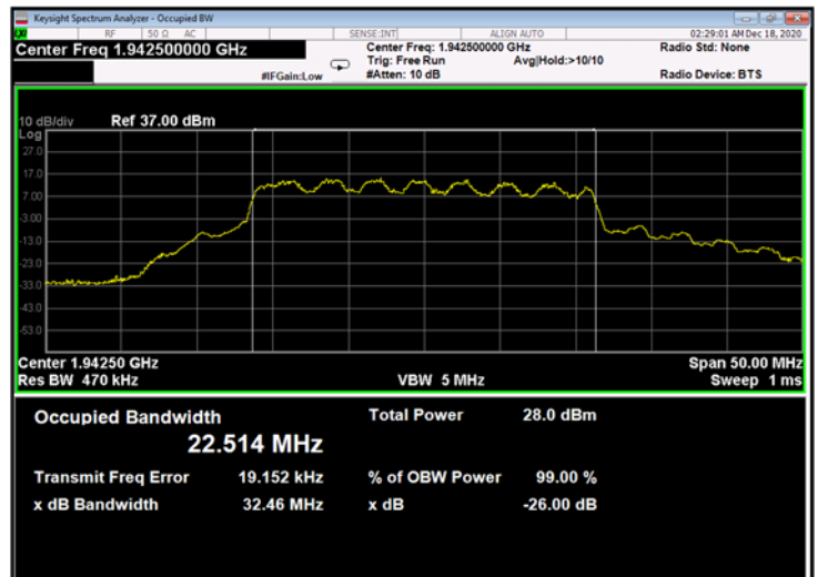
Figure 572: 16QAM 25MHz B.W.; 1942.5MHz, 60kHz - Output
