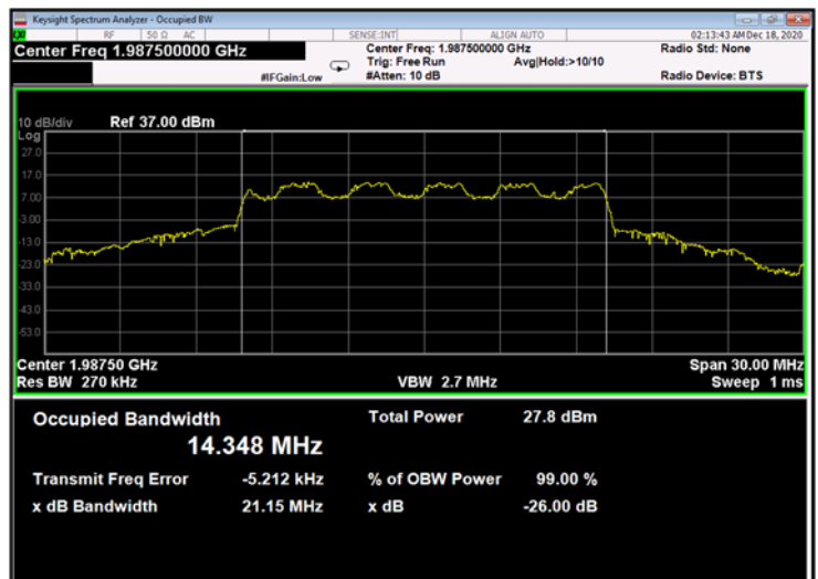
Figure 558: 16QAM 15MHz B.W.; 1987.5MHz, 15kHz - Output
