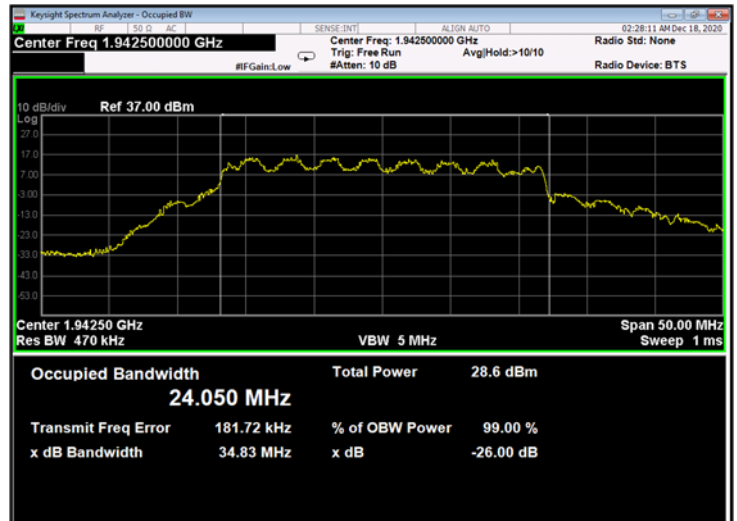
Figure 570: 16QAM 25MHz B.W.; 1942.5MHz, 15kHz - Output
