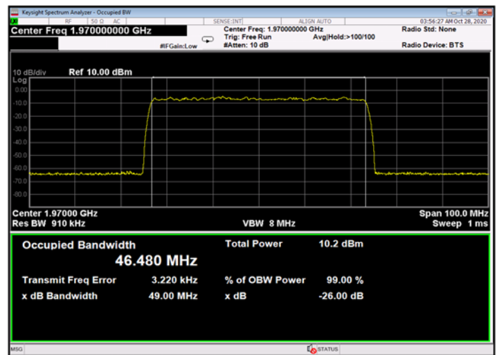
Figure 464: 256QAM 50MHz B.W.; 1970.0MHz, 60kHz - Input
