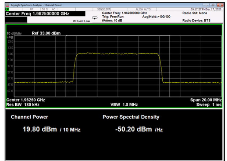
Figure 86: 64QAM 10MHz B.W.; 1962.5MHz, 60kHz
