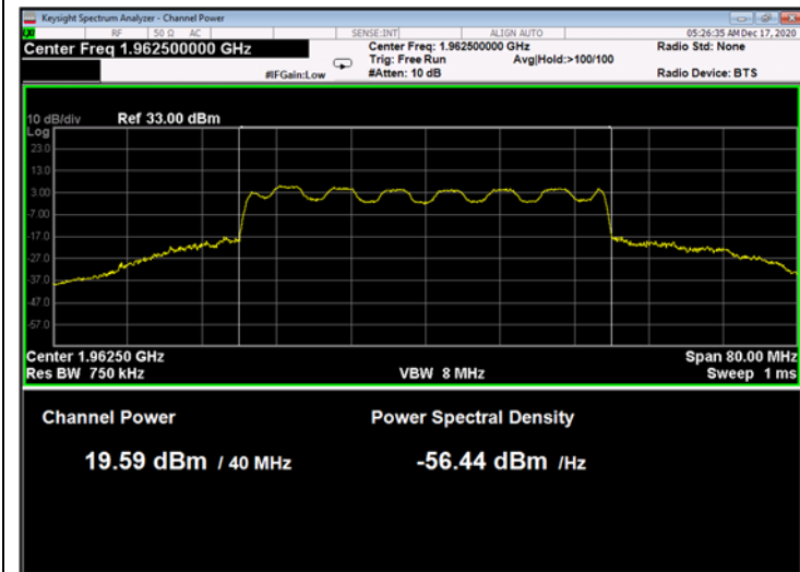
Figure 55: 16QAM 40MHz B.W.; 1962.5MHz, 30kHz
