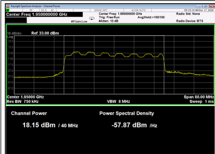
Figure 51: 16QAM 40MHz B.W.; 1950.0MHz, 15kHz
