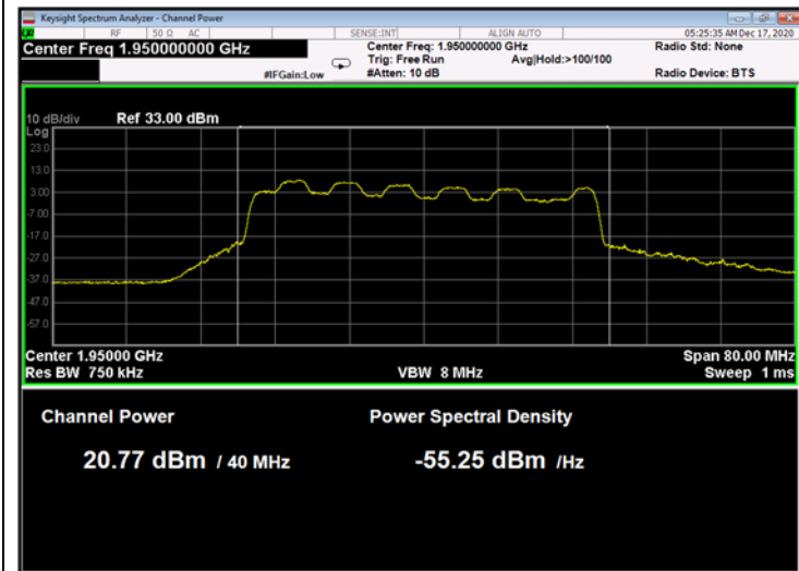
Figure 53: 16QAM 40MHz B.W.; 1950.0MHz, 60kHz
