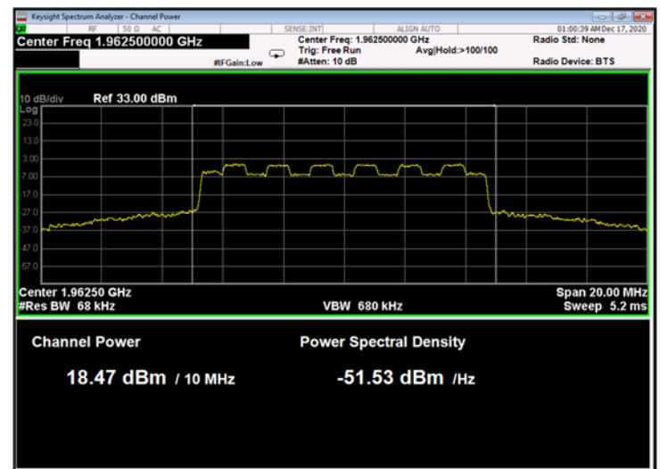
Figure 18: 16QAM 10MHz B.W.; 1962.5MHz, 15kHz
