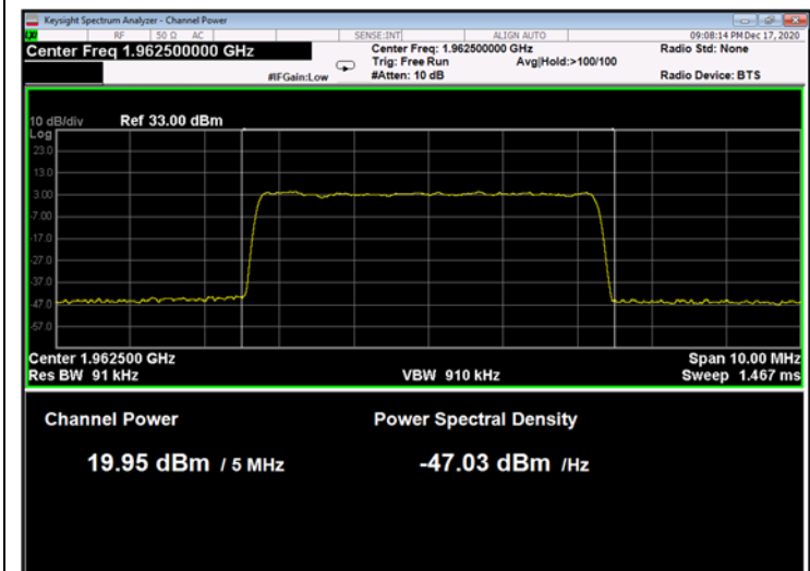
Figure 77: 64QAM 5MHz B.W.; 1962.5MHz, 15kHz
