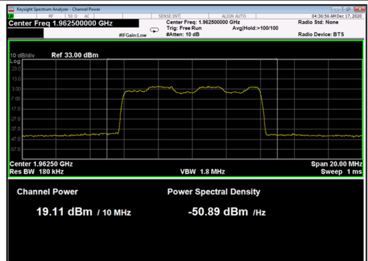
Figure 20: 16QAM 10MHz B.W.; 1962.5MHz, 60kHz
