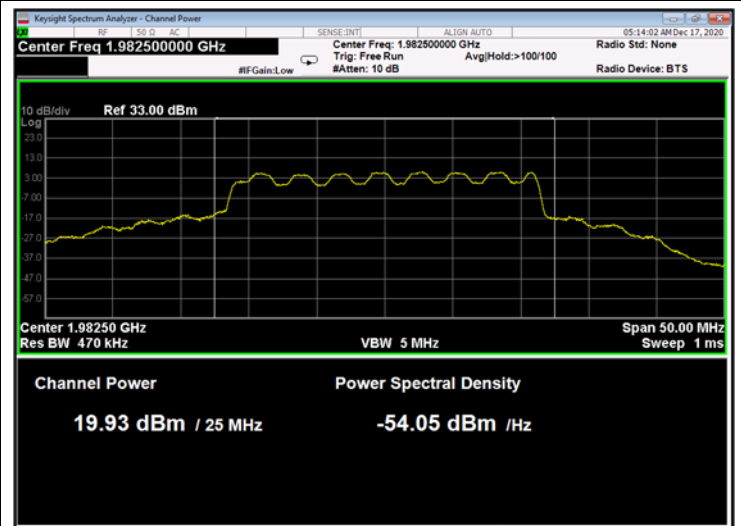
Figure 50: 16QAM 25MHz B.W.; 1982.5MHz, 60kHz
