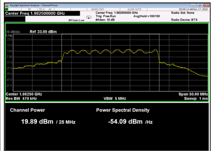
Figure 48: 16QAM 25MHz B.W.; 1982.5MHz, 15kHz
