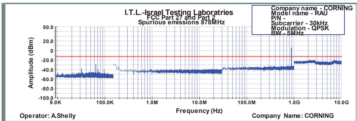
Figure 642: Spurious Emissions at Antenna Terminal QPSK 5MHz B.W.; 878.0MHz, 30kHz
