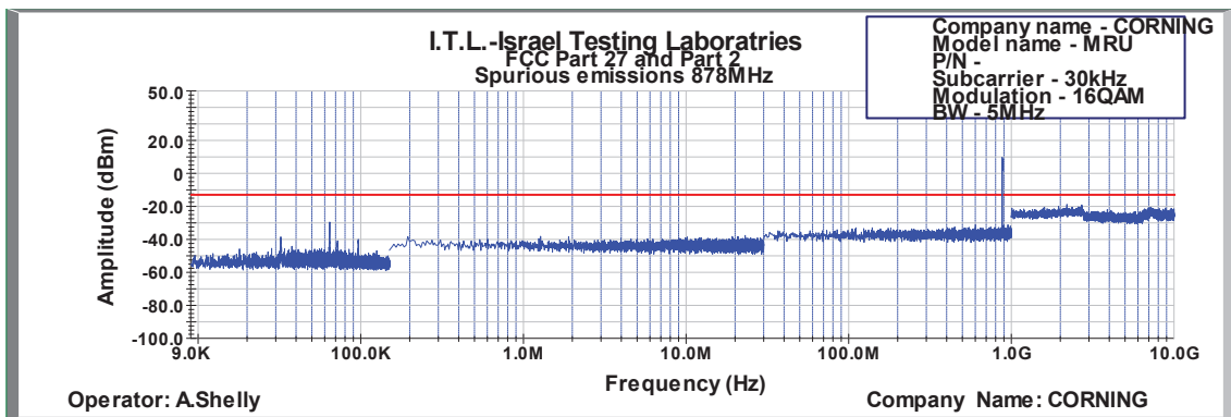
Figure 516: Spurious Emissions at Antenna Terminal 16QAM 5MHz B.W.; 878MHz, 30kHz
