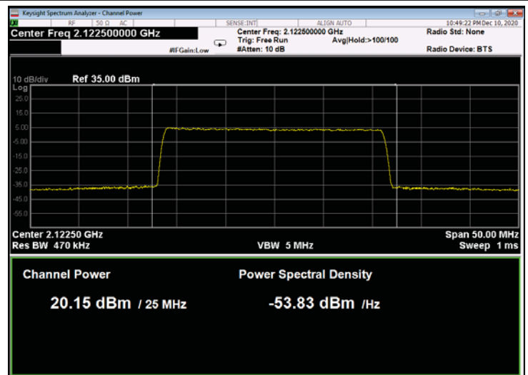
Figure 176: 256QAM 25MHz B.W.; 2122.5MHz, 60kHz
