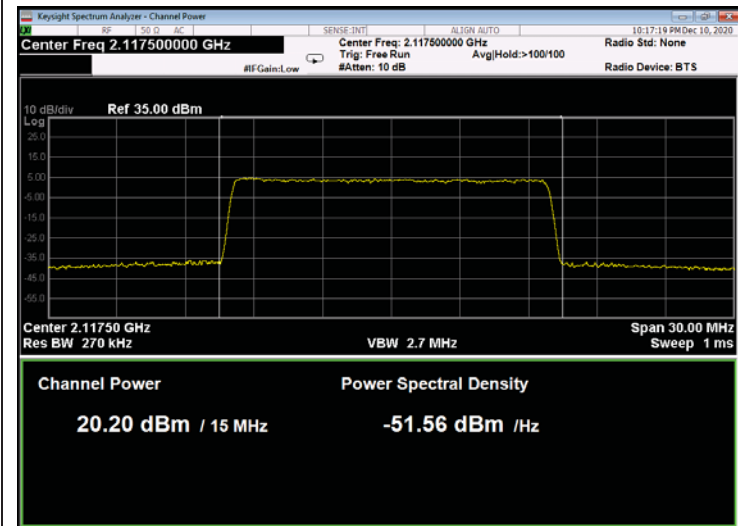
Figure 157: 256QAM 15MHz B.W.; 2117.5MHz, 30kHz
