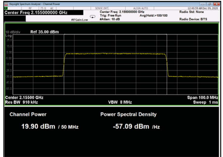
Figure 132: 64QAM 50MHz B.W.; 2155.0MHz, 15kHz
