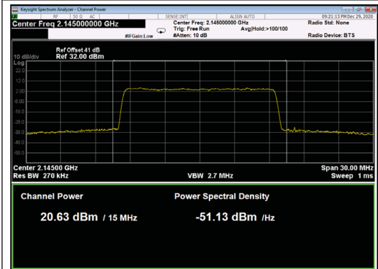
Figure 161: 256QAM 15MHz B.W.; 2145.0MHz, 60kHz
