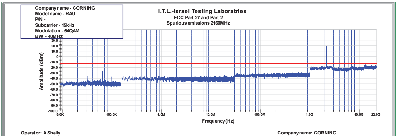
Figure 911: Spurious Emissions at Antenna Terminal 64QAM 40MHz B.W.; 2160.0MHz, 15kHz
